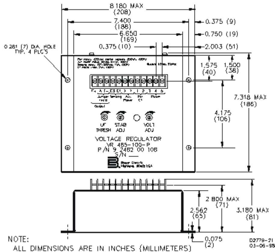
Figure 2-1. Outline Drawing
