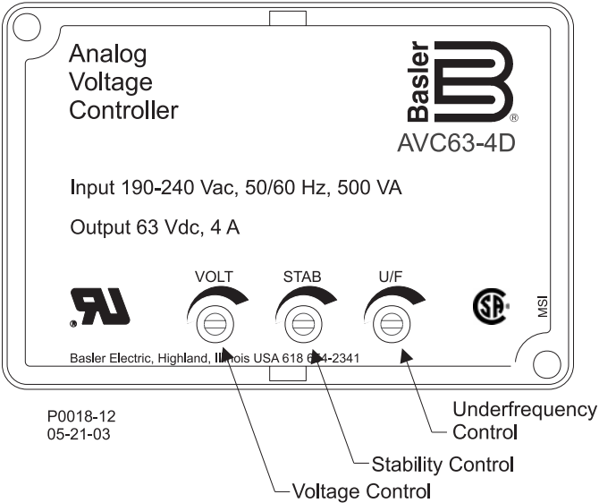
Figure 5 - AVC63-4D Potentiometer Control Locations
