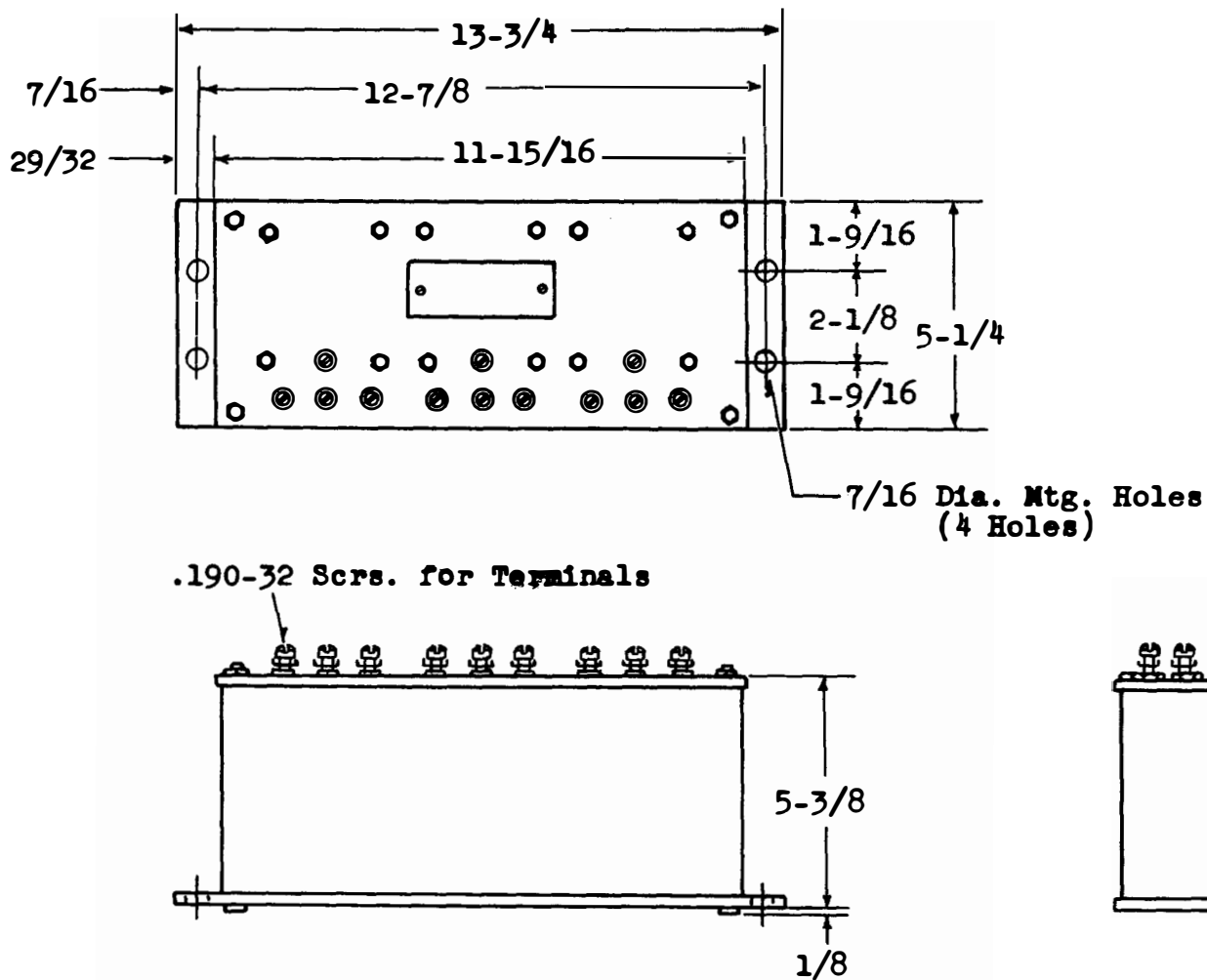
Figure 2 Outline and drilling plan of the three phase star-delta auxiliary current transformer.
