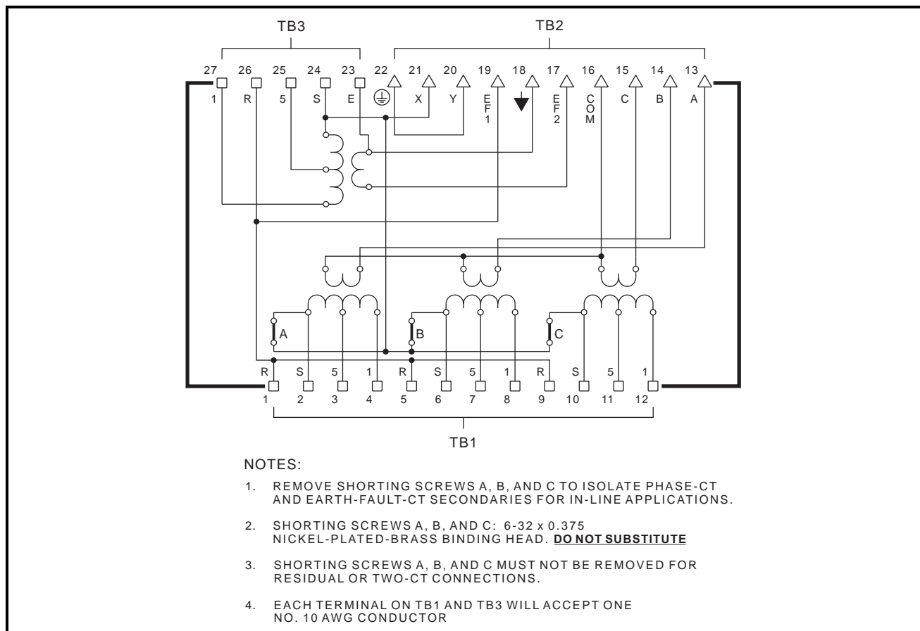
FIGURE 3.5 MPU-CIM Schematic.
