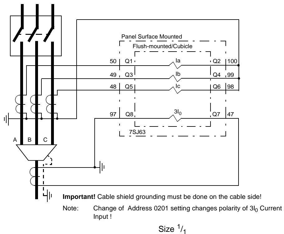
Figure A-37 Current connections to three current transformers and a core balance neutral current transformer for ground current – preferred for effectively or low-resistance grounded networks
