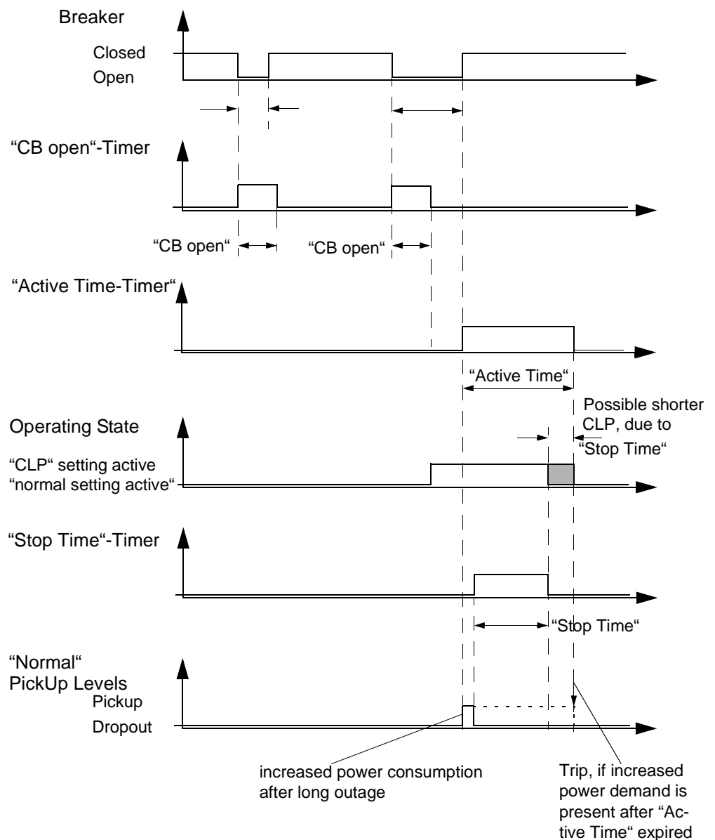
Figure 6-29 Cold Load Pickup Timing Sequence
