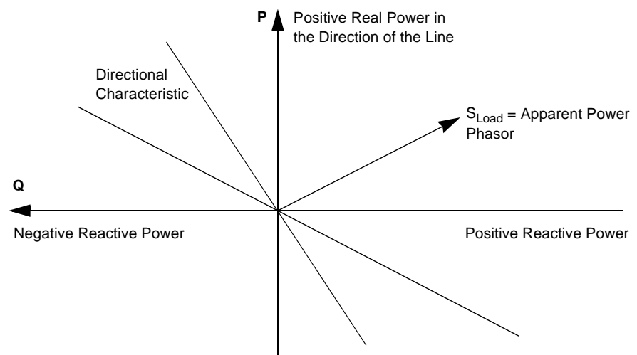
Figure 8-13 Apparent Power
