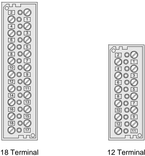
Figure 2-5 Terminal Blocks of Threaded Terminals for Voltage Connections — Rear View
