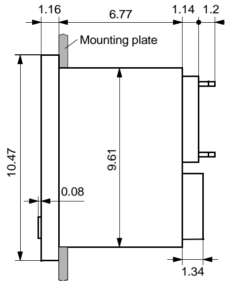
Side view (with clamp terminals)
