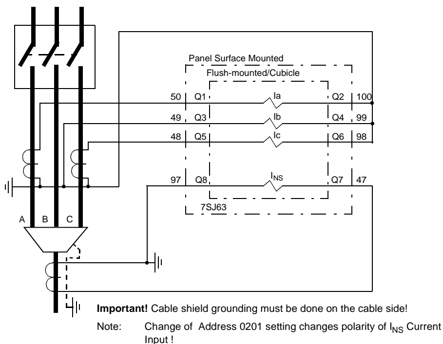
Figure A-38 Current connections to two current transformers and a core balance neutral current transformer for sensitive ground fault detection – only for ungrounded or compensated networks
