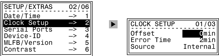
Figure 4-26 Readout of Time Synchronization Settings from the HMI
