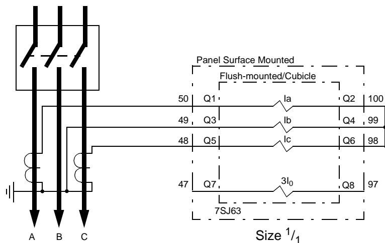
Figure A-36 Current connections to two current transformers - only for ungrounded or compensated networks.
