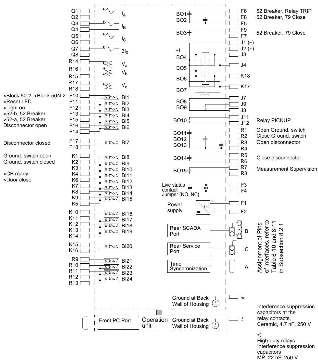
Figure A-14 General diagram 7SJ632*—*A/C (devices with separate operation unit) – V4.1 –
