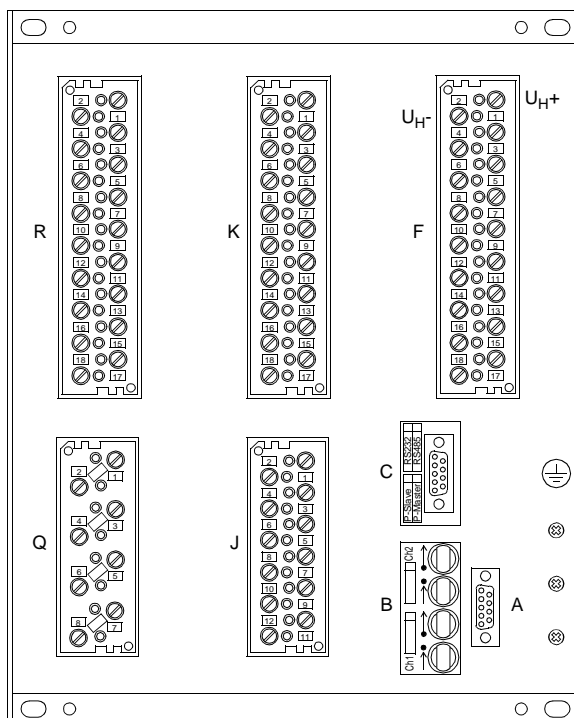
Figure 2-3 Rear View of a 7SJ63, Housing Size \frac{1}{2} with Screw-type Terminals (example only)
