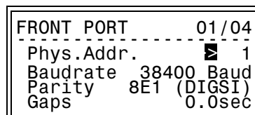
Figure 5-53 Reading and Setting the Front DIGSI Port at the Device Controls
