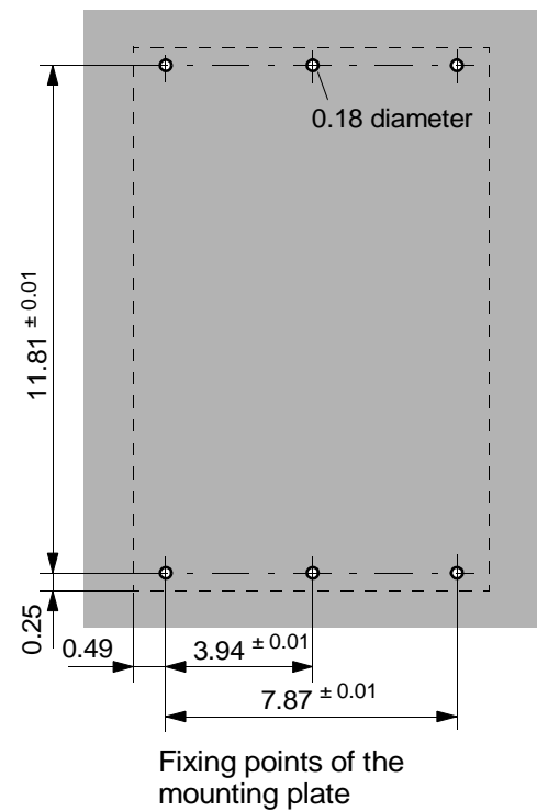
Figure 10-11 Dimensions 7SJ63 (size \frac{1}{2} ) for devices with detached operator panel
