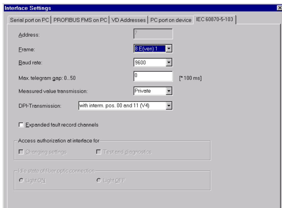
Figure 4-27 DIGSI® 4, Interface Settings Window
