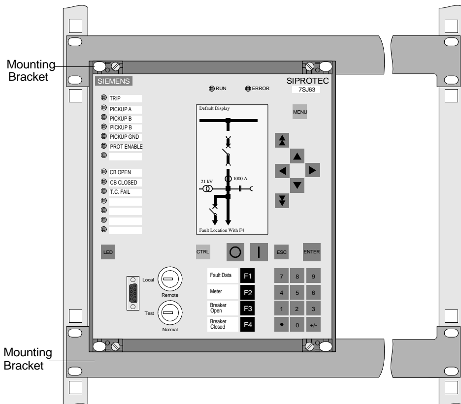
Figure 8-3 Installing a 7SJ63 with \frac{1}{2} Size Housing in a Rack
