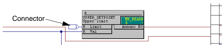
Figure 5-39 Connector
