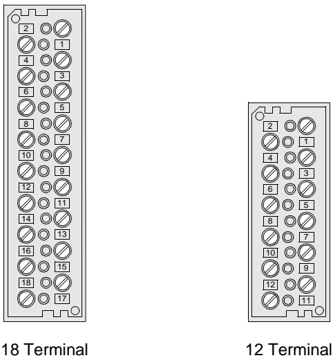
Figure 2-22 Terminal Blocks of Threaded Terminals for Voltage Connections — Rear View
