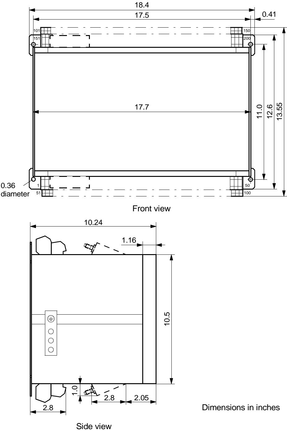
Figure 10-10 Dimensions 7SJ63 for panel surface mounting (size 1 1/4)
