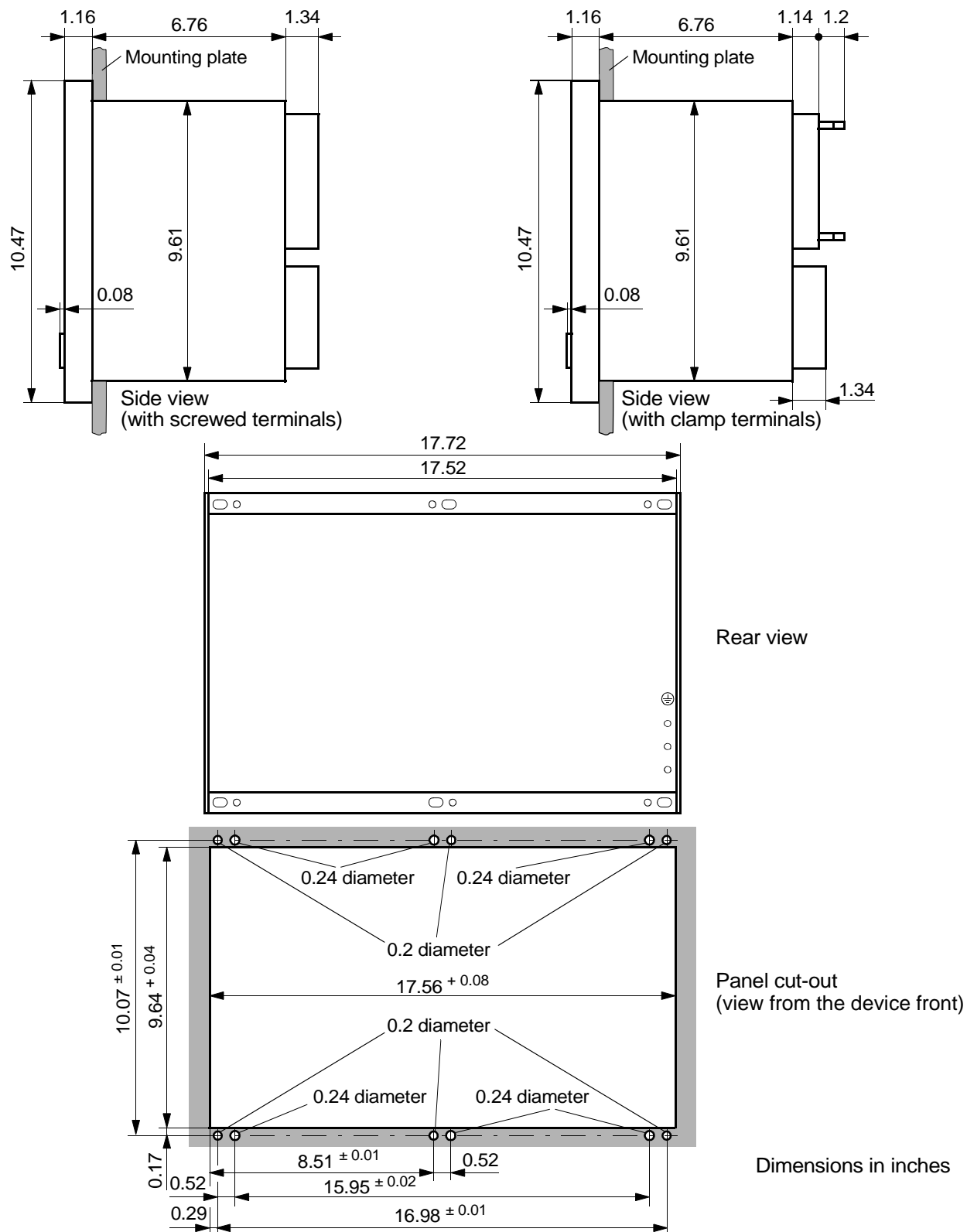
Figure 10-8 Dimensions 7SJ63 for panel flush mounting or cubicle installation (size \frac{1}{4} )
