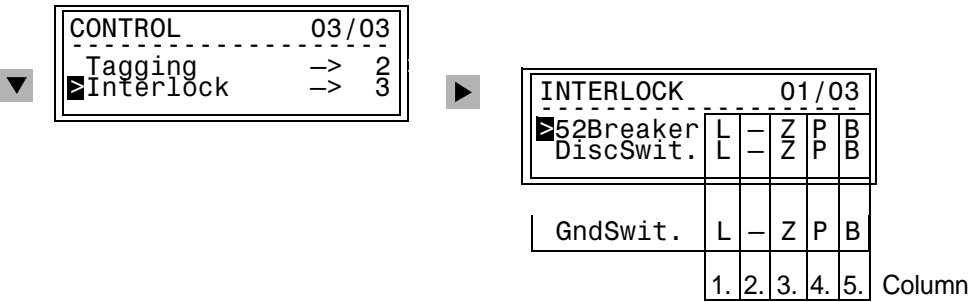
Figure 7-51 Example of Interlocking Conditions for Switching Equipment, Front Panel
