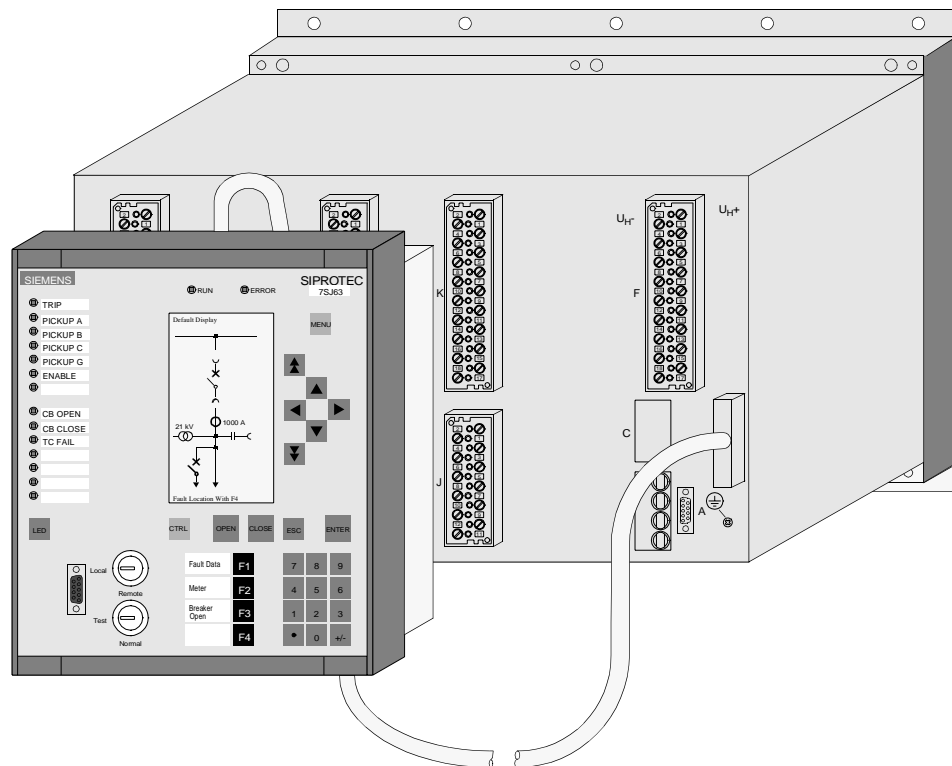
Figure 2-21 7SJ63, Detached Operator Panel, Threaded Terminals (Housing Size 1\frac{1}{4} )
