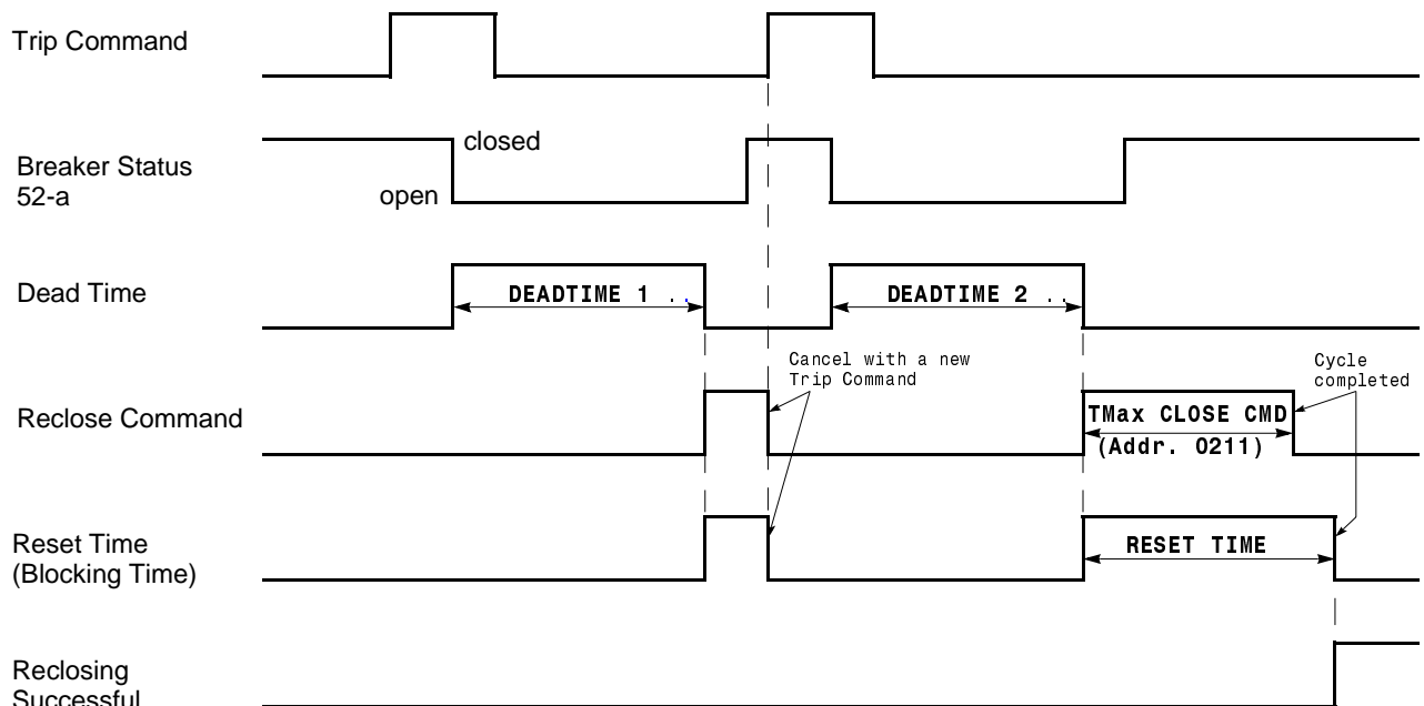
Figure 6-56 Timing Diagram for a Second Successful Reclosure
