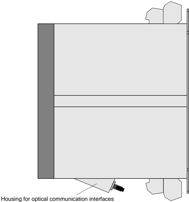
Figure 2-18 Side View of 7SJ63, Panel Surface-mounting, Optical Communication Interface
