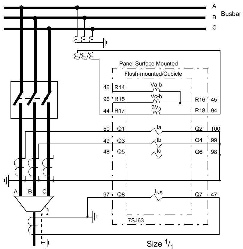
Figure A-42 Current and voltage connections to three current transformers, core balance neutral current transformers and open delta voltage transformers, maximum precision for sensitive ground fault detection.
