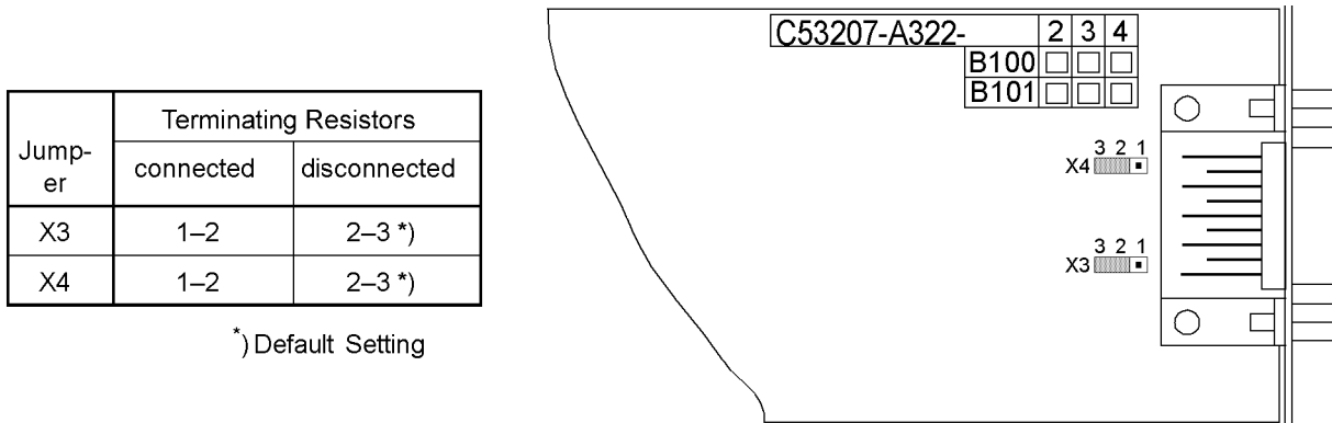
Figure 3-17 Position of the plug-in jumpers for the configuration of the terminating resistors at the interfaces Profibus (FMS and DP) and DNP3.0 interface
