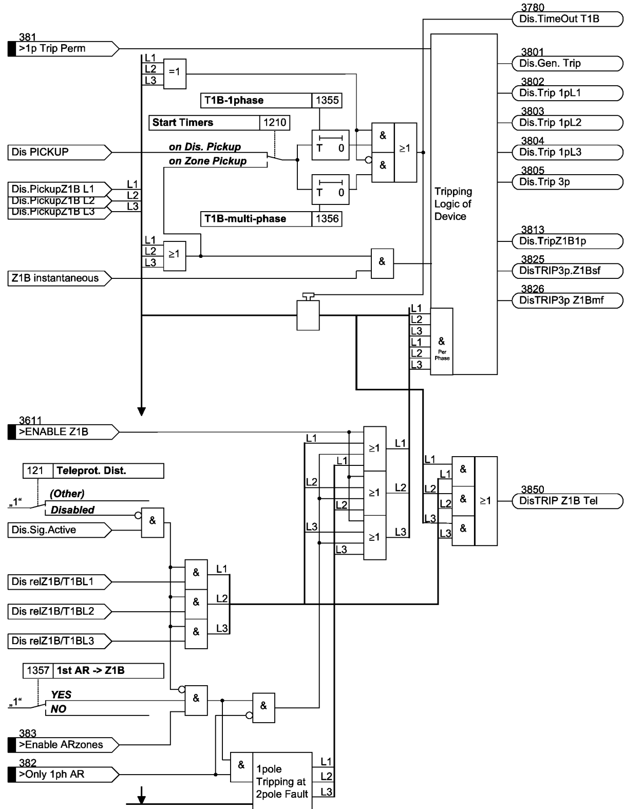
Figure 2-32 Tripping logic for the controlled zone Z1B
