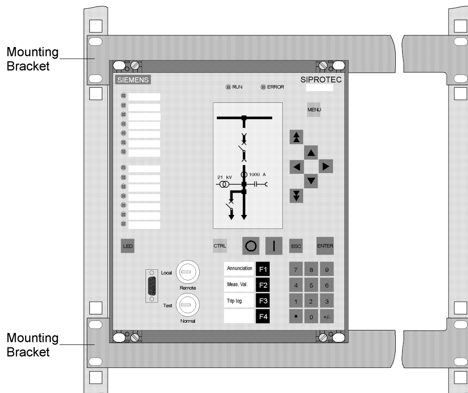
Figure 3-25 Installation example of a unit in a rack or cubicle (housing size \frac{1}{2} )
