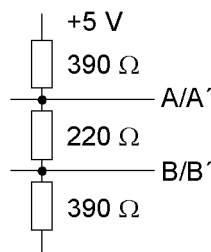
Figure 3-18 Termination of the RS485 interface (external)
