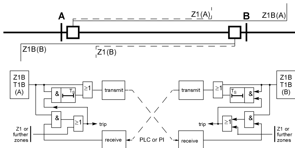
Figure 2-49 Function diagram of the permissive overreach transfer trip method
