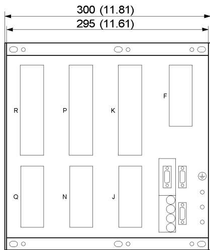
Rear View
