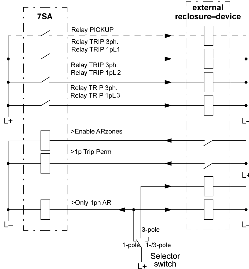
Figure 2-112 Connection example with external auto-reclosure device for 1-/3-pole AR with mode selector switch
