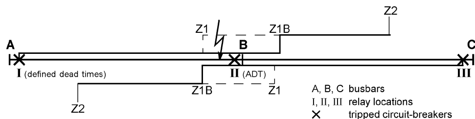
Figure 2-110 Example of adaptive dead time (ADT)
