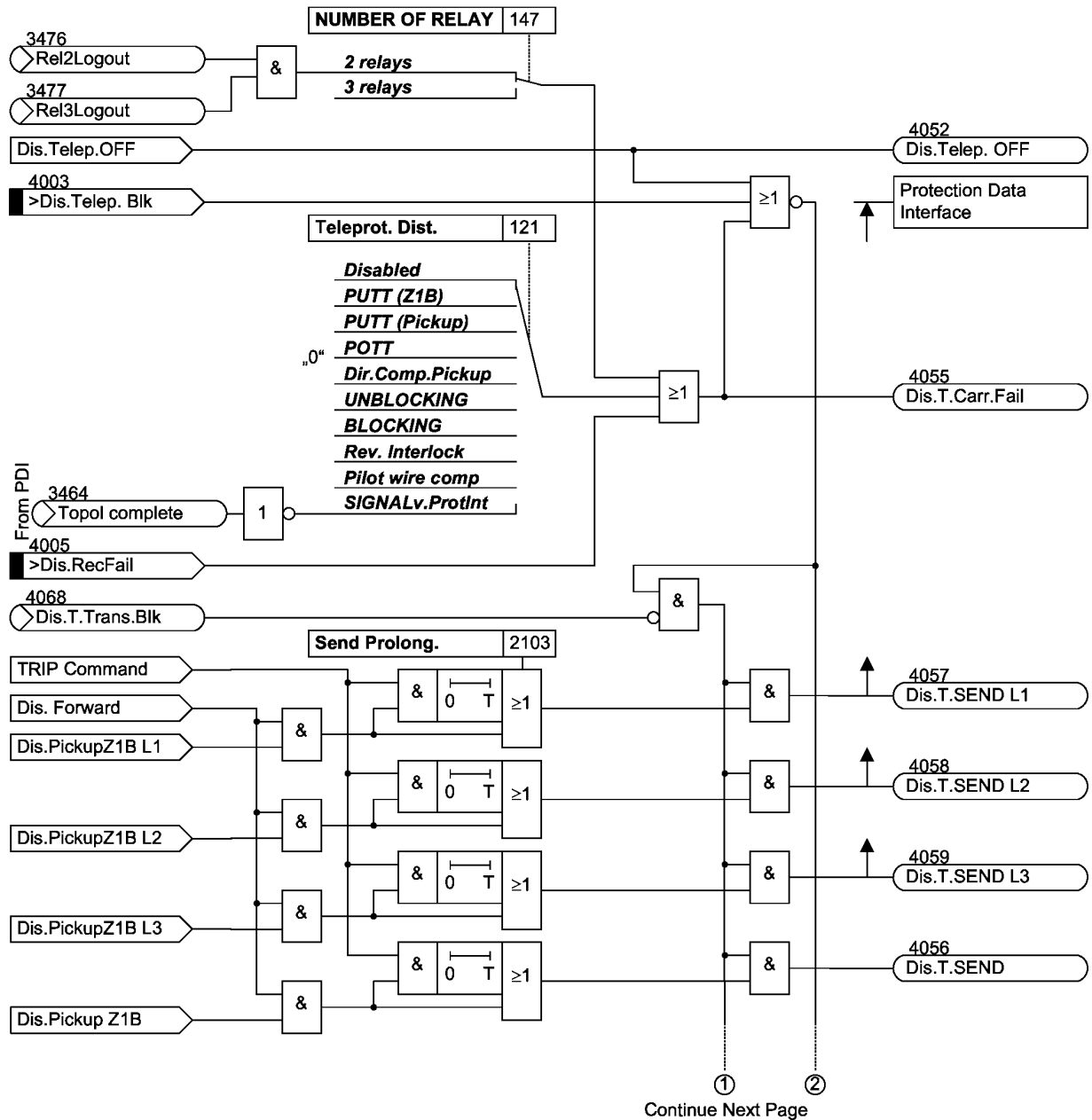
Figure 2-51 Logic diagram of the permissive overreach transfer trip (POTT) scheme (one line end, with protection data interface)
