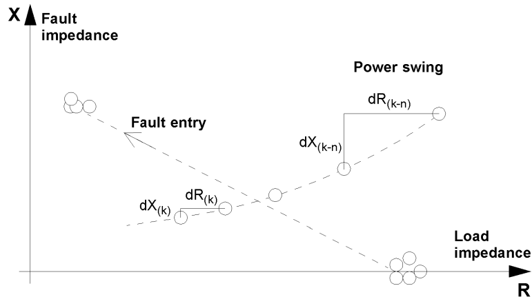
Figure 2-35 Impedance vector during power swing
