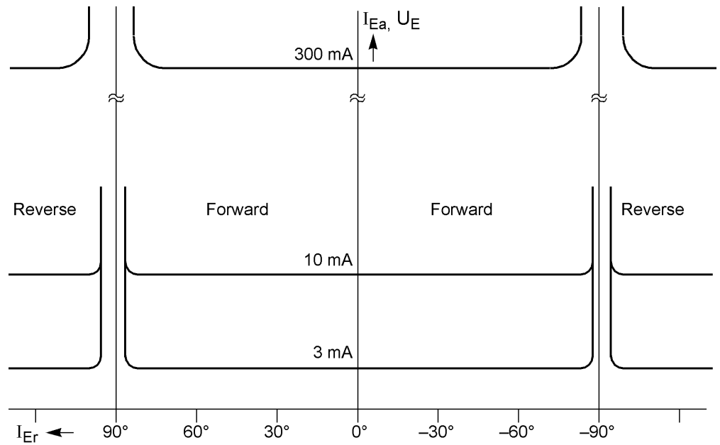
Figure 2-103 Measurement characteristic of the sensitive direction determination for earth fault in a resonant-earthed system
