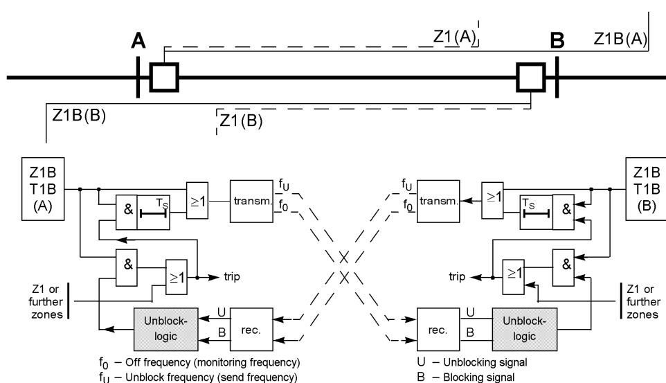
Figure 2-55 Function diagram of the directional unblocking method
