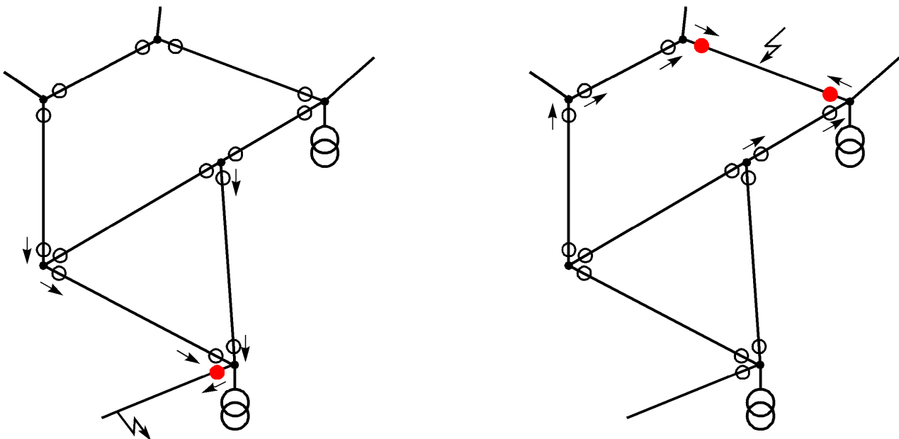
Figure 2-105 Faulted line location in meshed networks using directional indications
