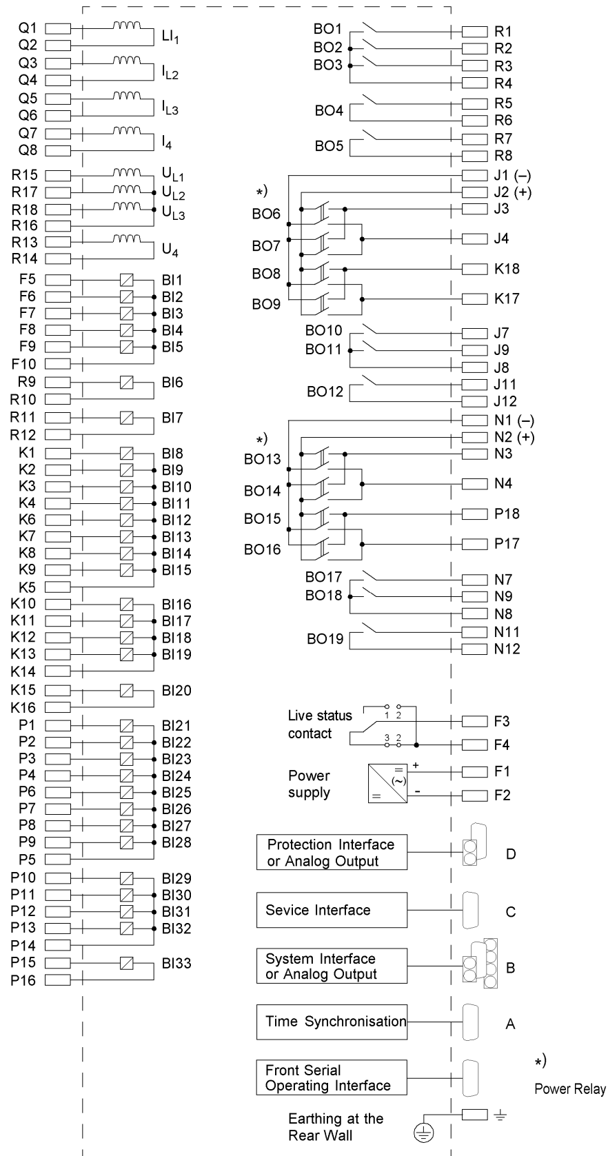
Figure A-10 General diagram for 7SA6*2*-*C/L (panel flush mounting or cubicle mounting)
