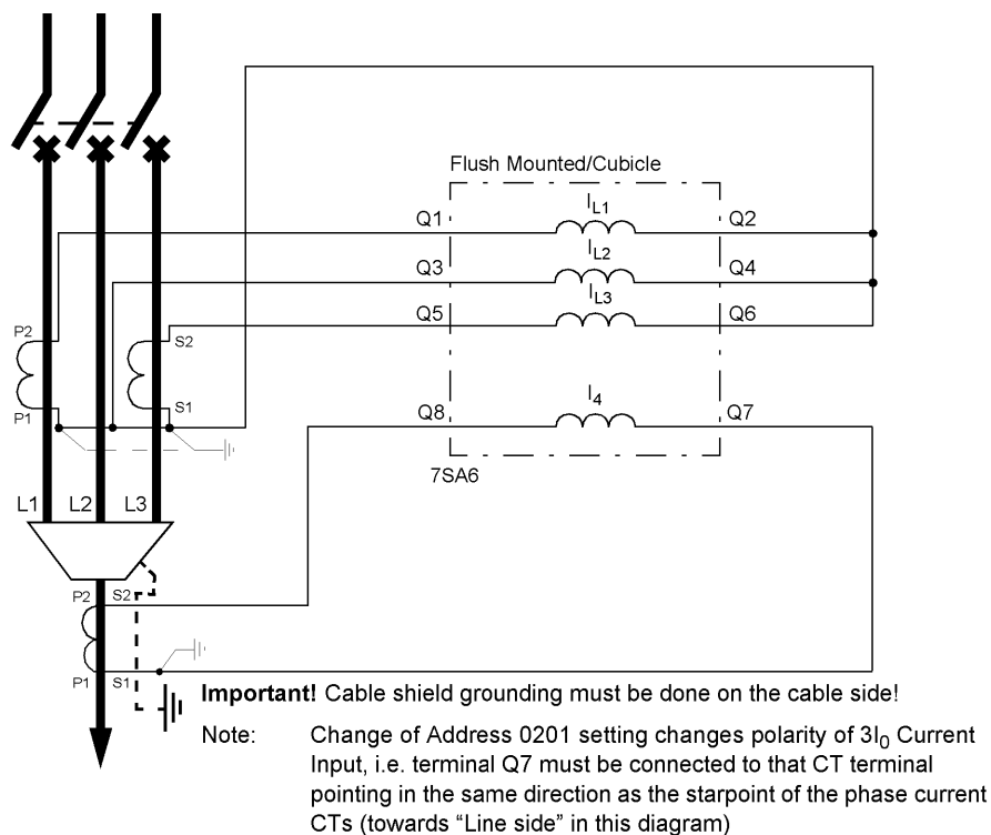
Figure A-35 Current connections to 2 current transformers with separate earth current transformer (summation current transformer or toroidal transformer) not permitted for earthed systems
