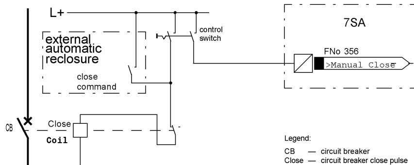
Figure 2-159 Manual closing with external automatic reclosure device
