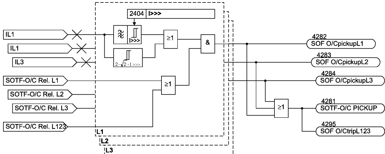
Figure 2-101 Logic diagram of the high current switch on to fault protection
