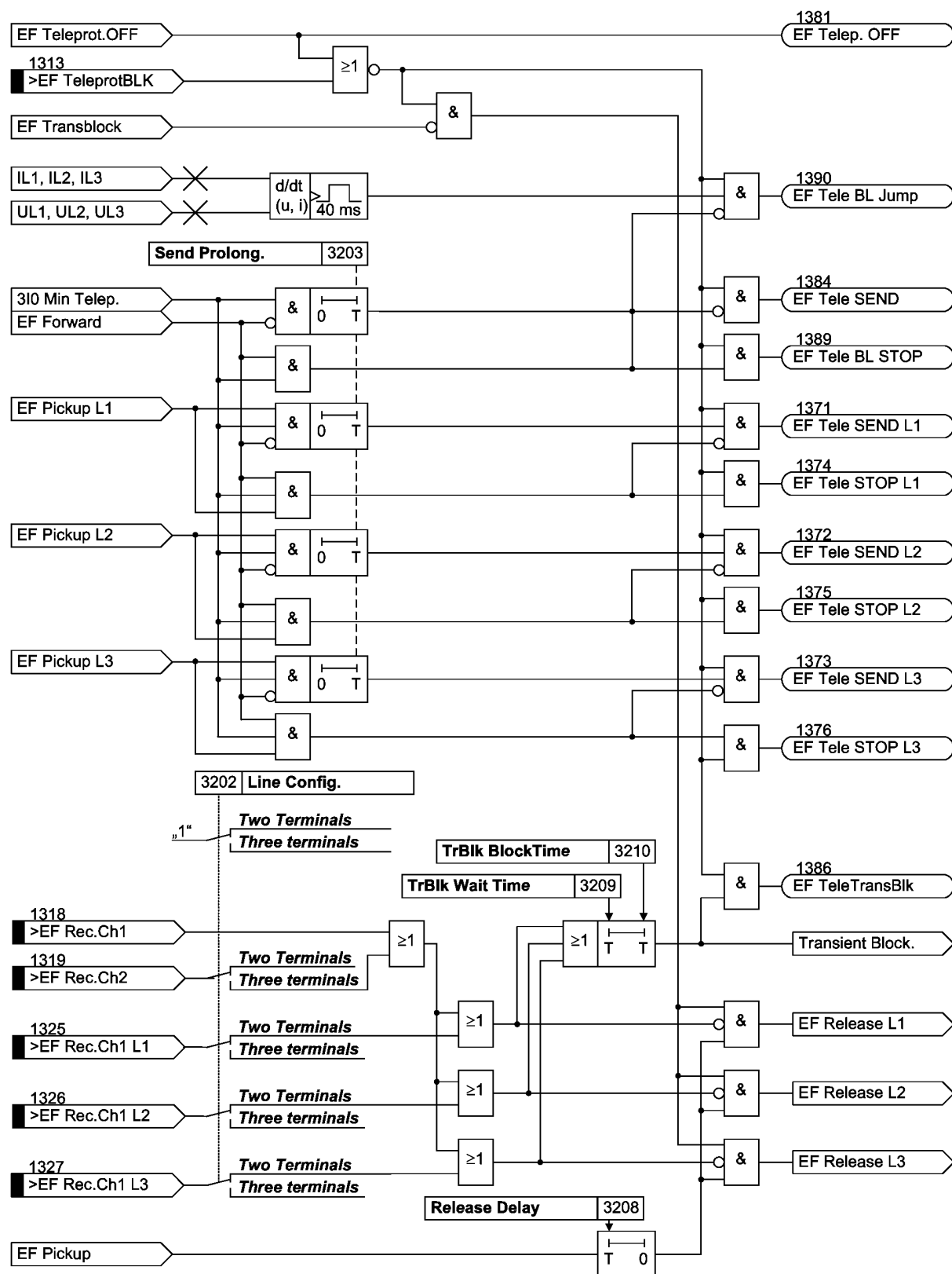
Figure 2-87 Logic diagram of the blocking scheme (one line end)
