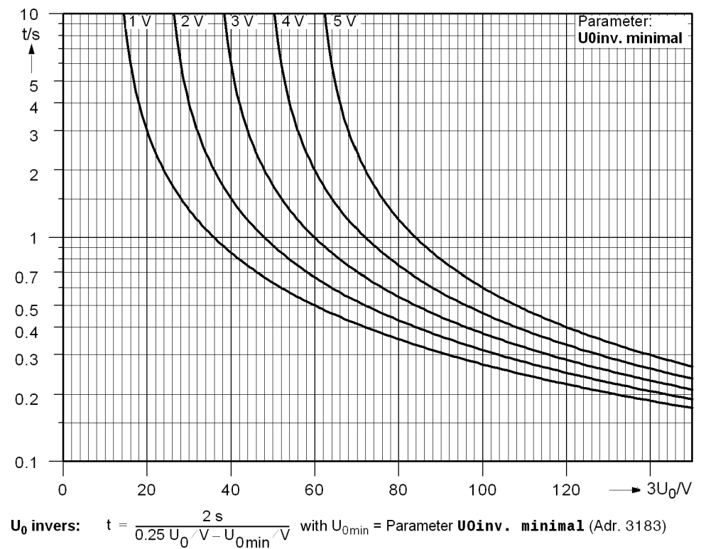
Figure 4-5 Trip time characteristics of the zero sequence voltage protection U_{0 \text{ inv.}}
