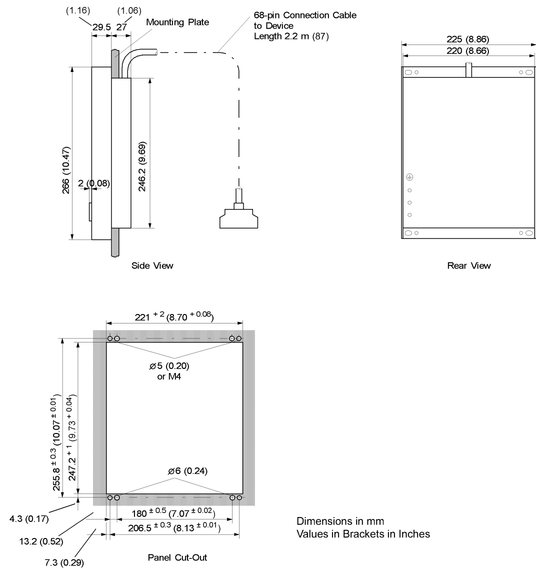
Figure 4-17 Dimensions of a Detached Operator Panel
