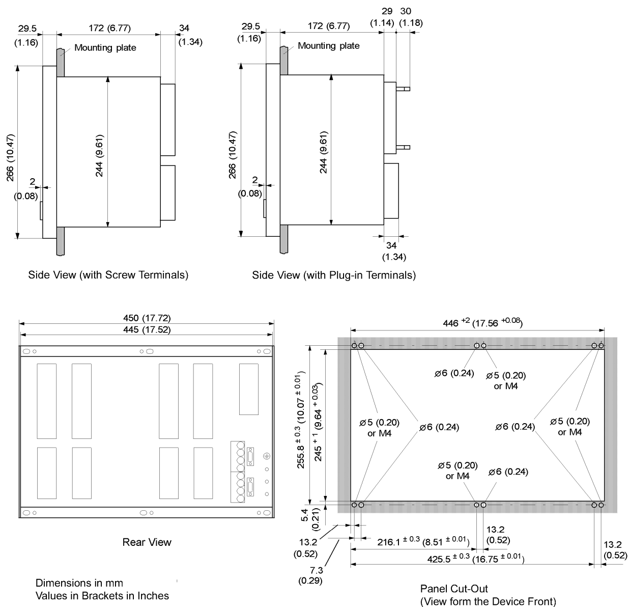
Figure 4-11 Dimensions of a device for panel flush or cubicle mounting (size 1/1 )
