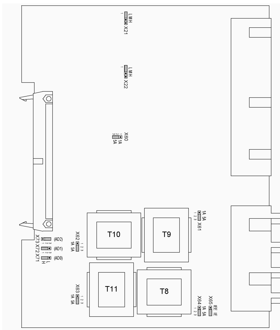
Figure 3-12 C-I/O-11 input/output board with representation of jumper settings required for checking configuration settings
