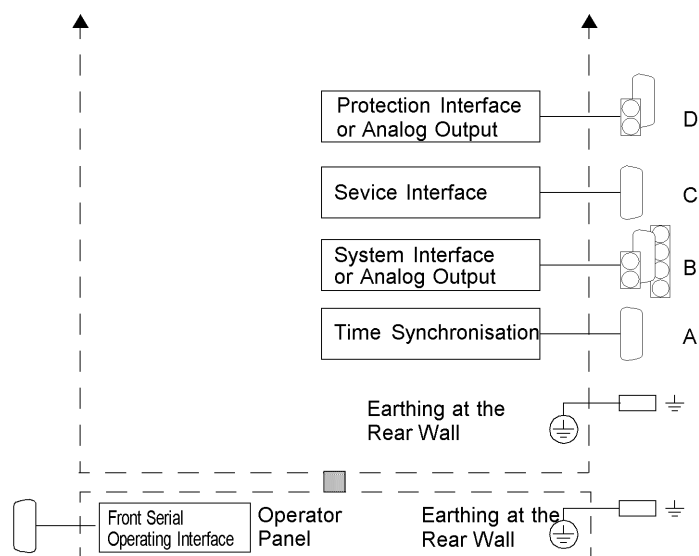
Figure A-27 General diagram 7SA642*-*B/K (panel surface mounting with detached operator panel)
