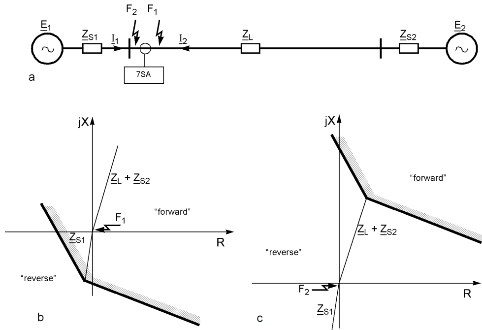
Figure 2-24 Directional characteristic with quadrature or memorized voltages
