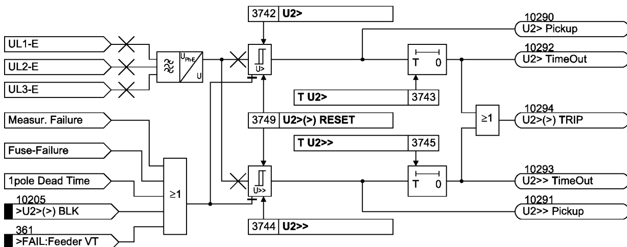
Figure 2-123 Logic diagram of the overvoltage protection for the negative sequence voltage system U_2
