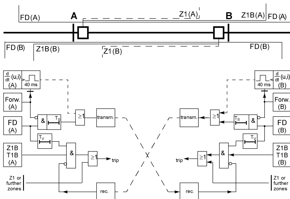
Figure 2-58 Function diagram of the blocking scheme
