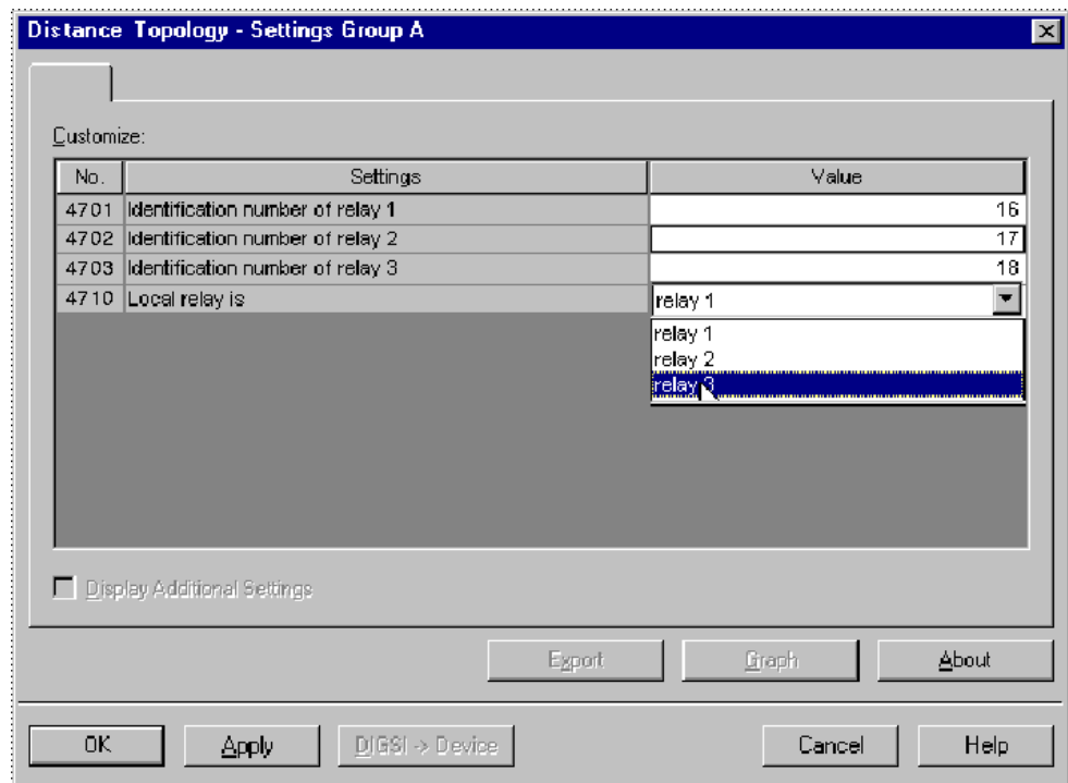
Figure 2-42 Distance protection topology for 3 ends with 3 devices - example
