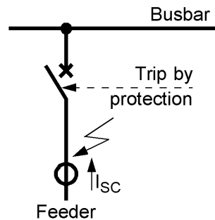
Figure 2-142 End fault between circuit breaker and current transformers
