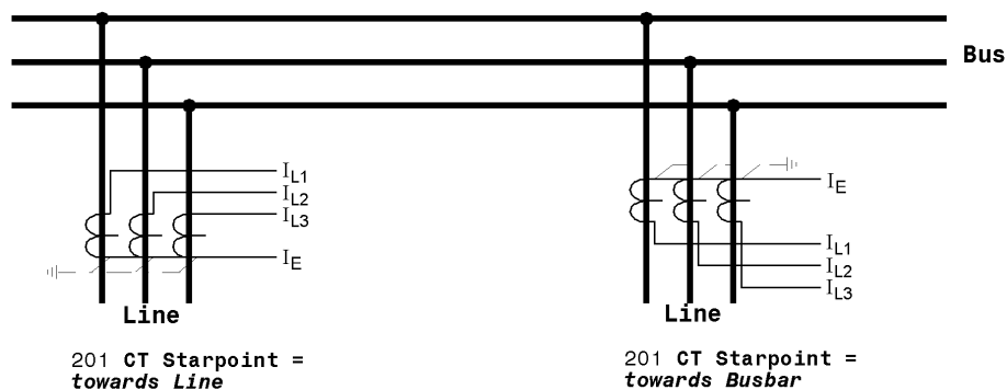
Figure 2-2 Polarity of Current Transformers
