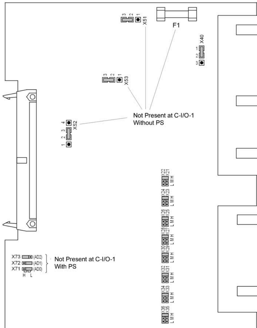
Figure 3-9 Input/output board C-I/O-1 with representation of the jumper settings required for the board configuration
