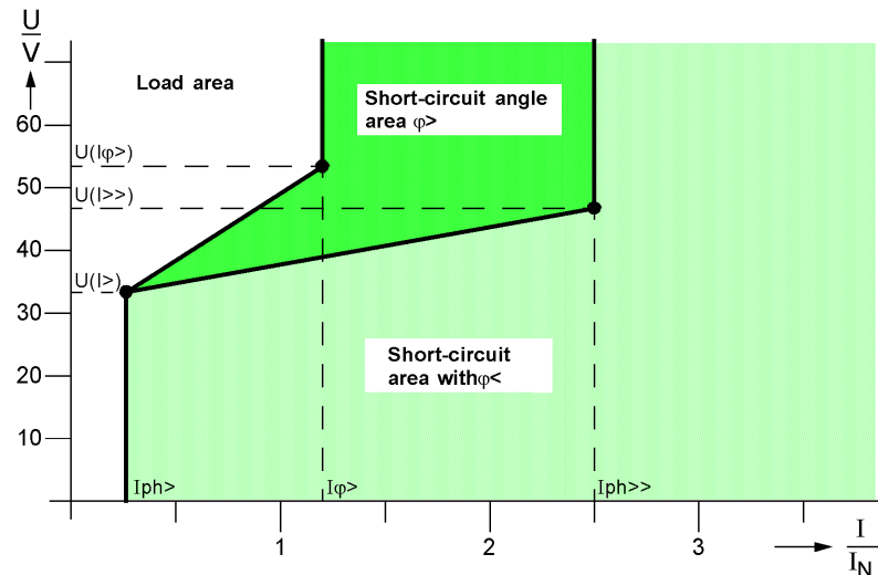
Figure 2-12 U/I/\varphi characteristic
