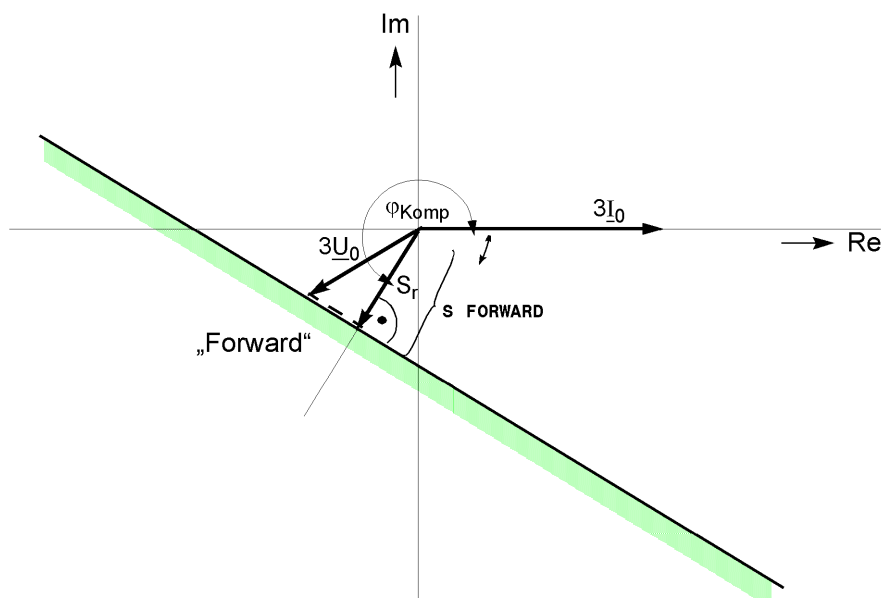
Figure 2-74 Directional characteristic with zero sequence power, example S_r = setting value S FORWARD
