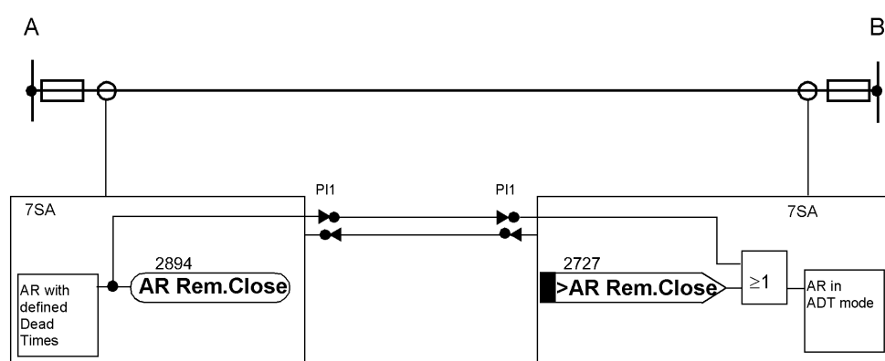
Figure 2-111 AR Remote-Close function via protection data interface
