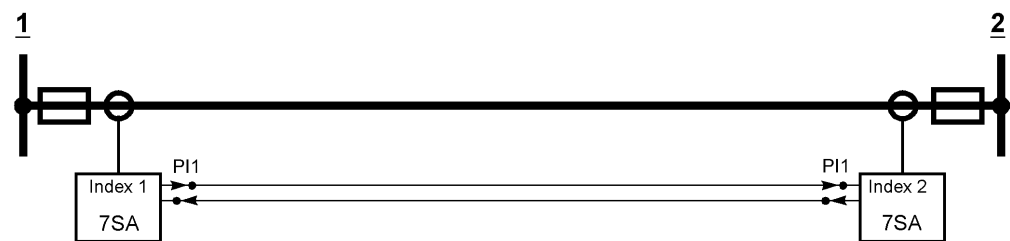
Figure 2-38 Distance protection for two ends with two 7SA6 devices with one protection data interface each (transmitter/ receiver)
