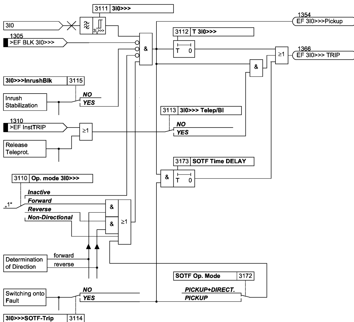
Figure 2-67 Logic diagram of the 3I_{0>>>} -stage
