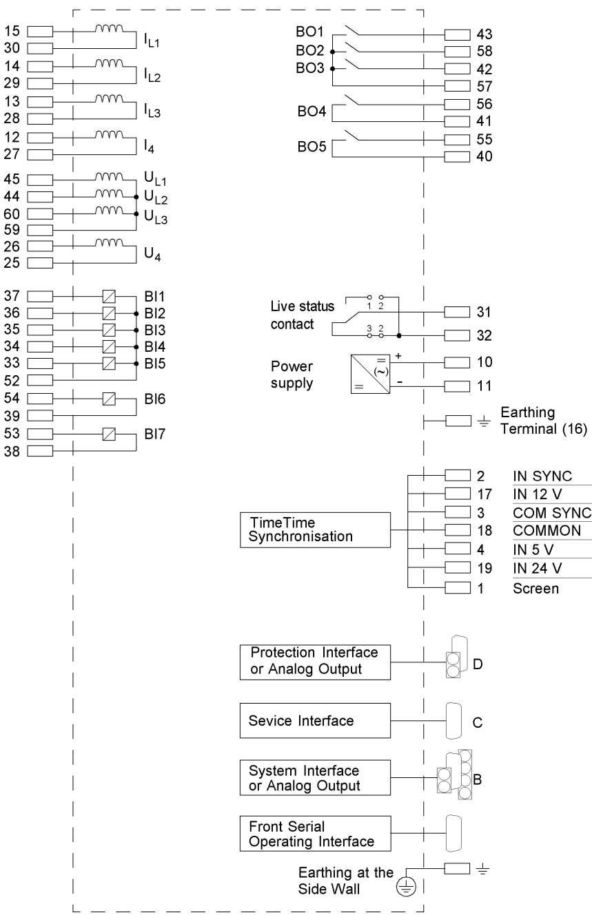
Figure A-14 General diagram for 7SA610*-*F (panel surface mounting)
