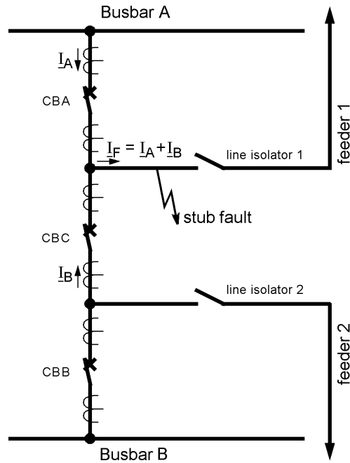
Figure 2-99 Stub fault at an 1 1/2 circuit breaker arrangement
