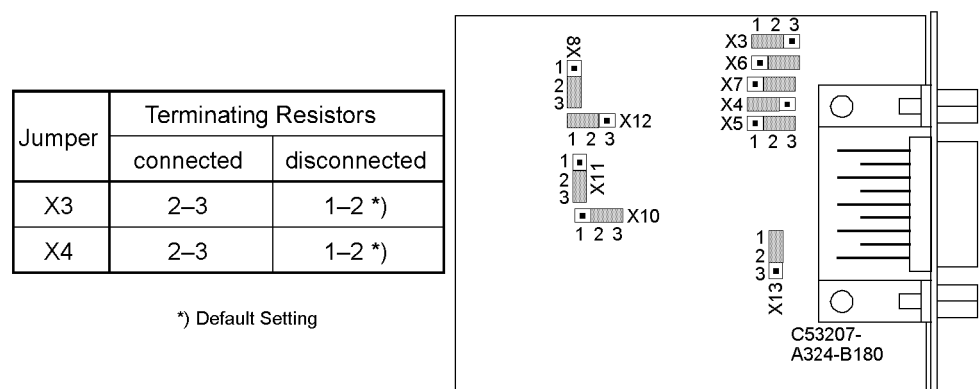
Figure 3-16 Position of terminating resistors and the plug-in jumpers for configuration of the RS485 interface
