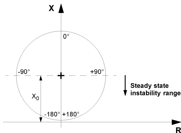
Figure 2-36 Steady state instability range
