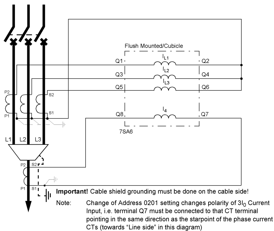
Figure A-33 Current connections to three current transformers with separate earth current transformer (summation current transformer or toroidal current transformer)
