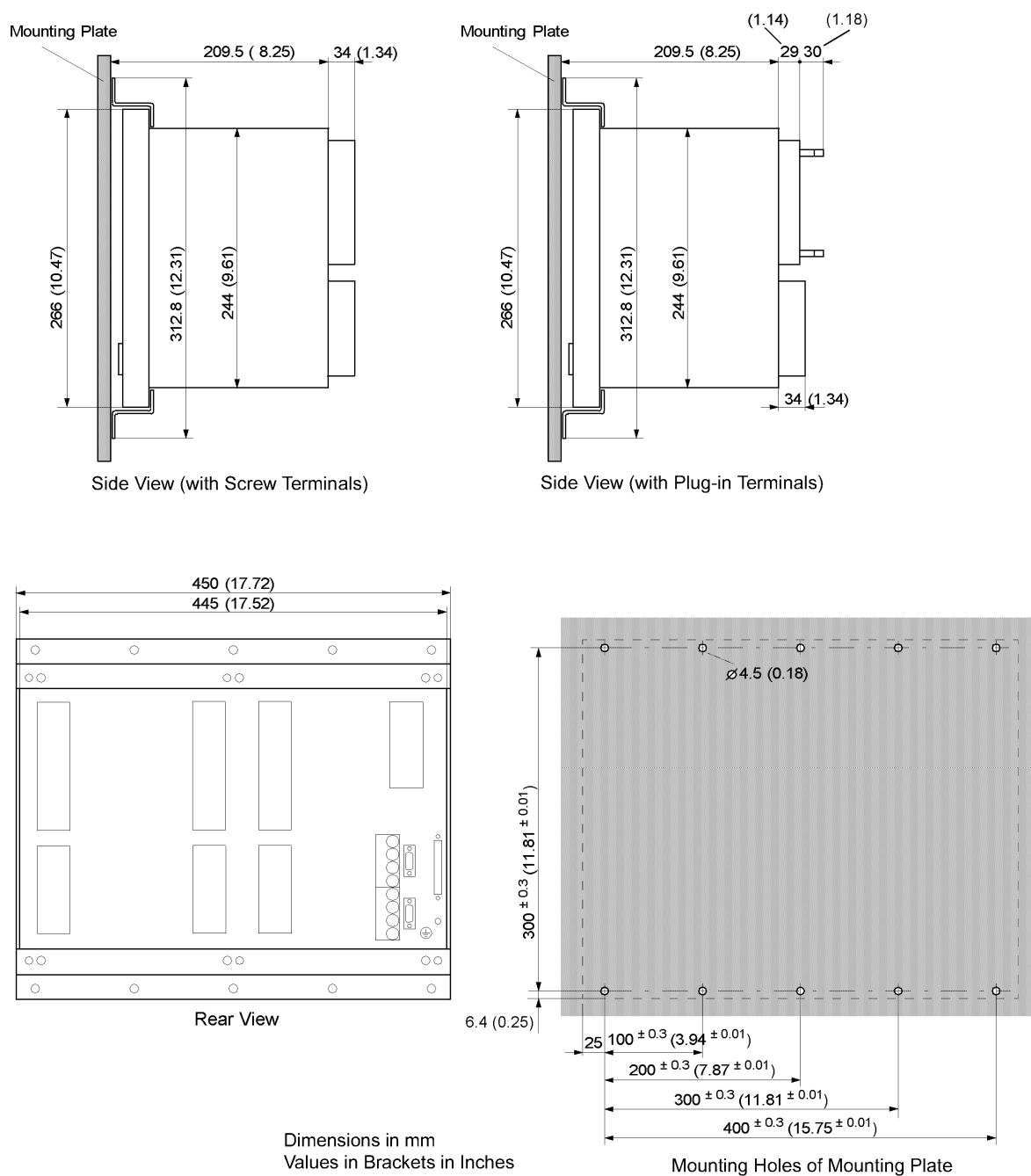
Figure 4-16 Dimensions of a device for surface mounting with detached operator panel (size 1 1 )
