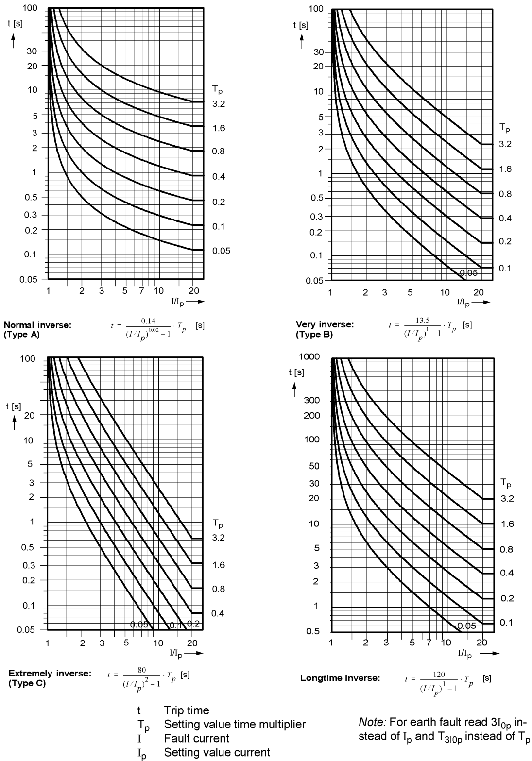
Figure 4-1 Trip time characteristics of inverse time overcurrent stage, acc. IEC (phases and earth)
