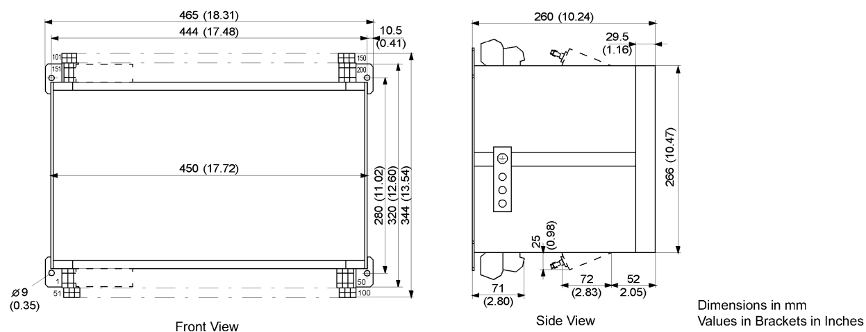
Figure 4-14 Dimensions of a device for panel surface mounting (size 1\frac{1}{4} )
