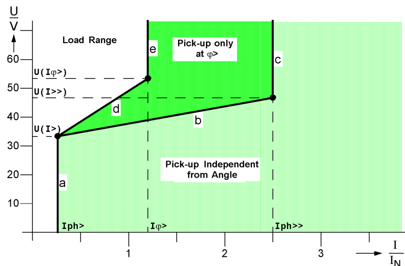
Figure 2-20 Parameters of the U/I/φ pickup
