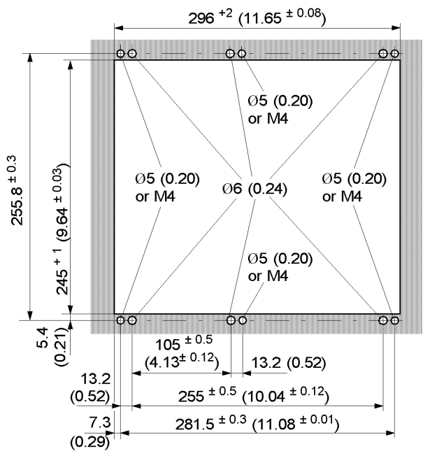
Panel Cut-Out
