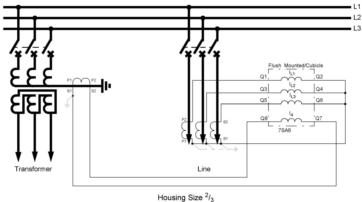
Figure A-39 Current connections to three current transformers and earth current from the star-point current of an earthed power transformer (for directional earth fault protection)
