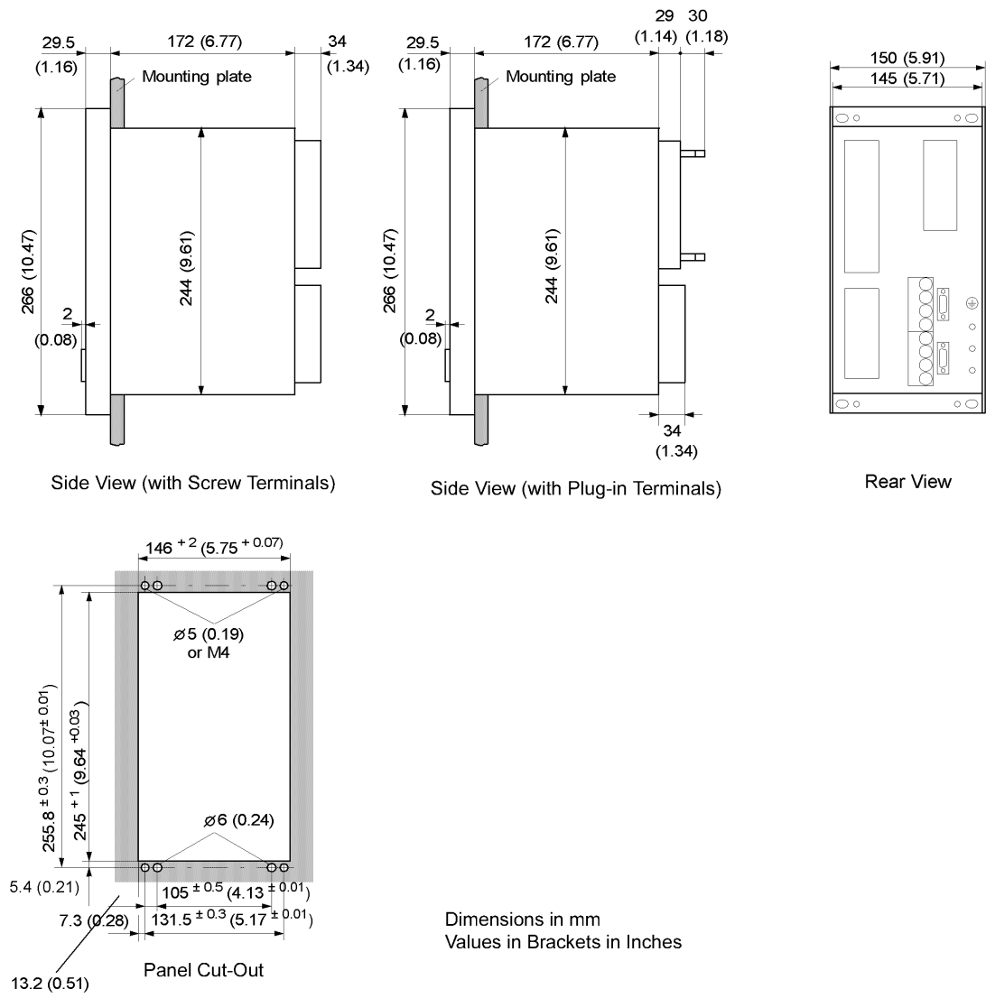
Figure 4-8 Dimensions of a device for panel flush mounting or cubicle installation (size 1/3)
