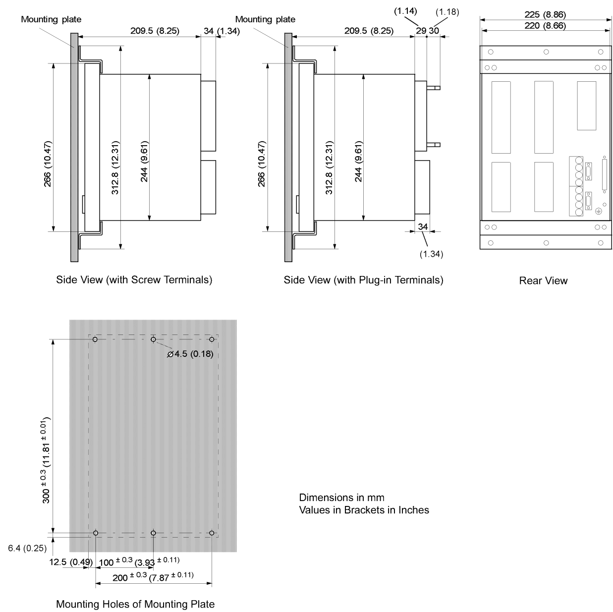
Figure 4-15 Dimensions of a device for surface mounting with detached operator panel (size 1/2)
