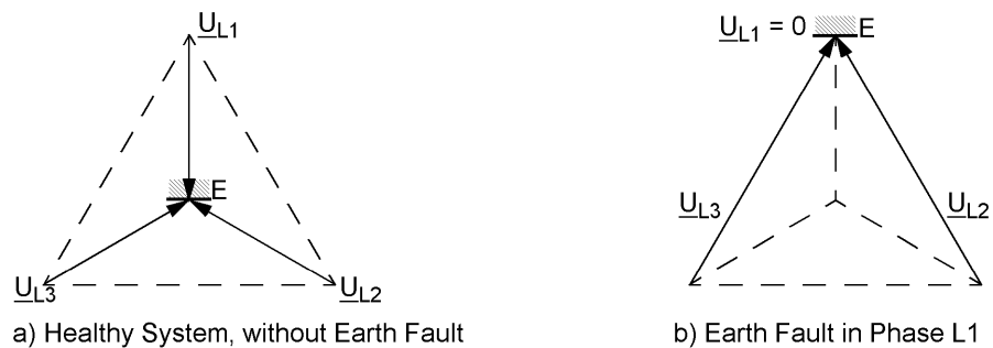
Figure 2-17 Earth fault in non-earthed neutral system
