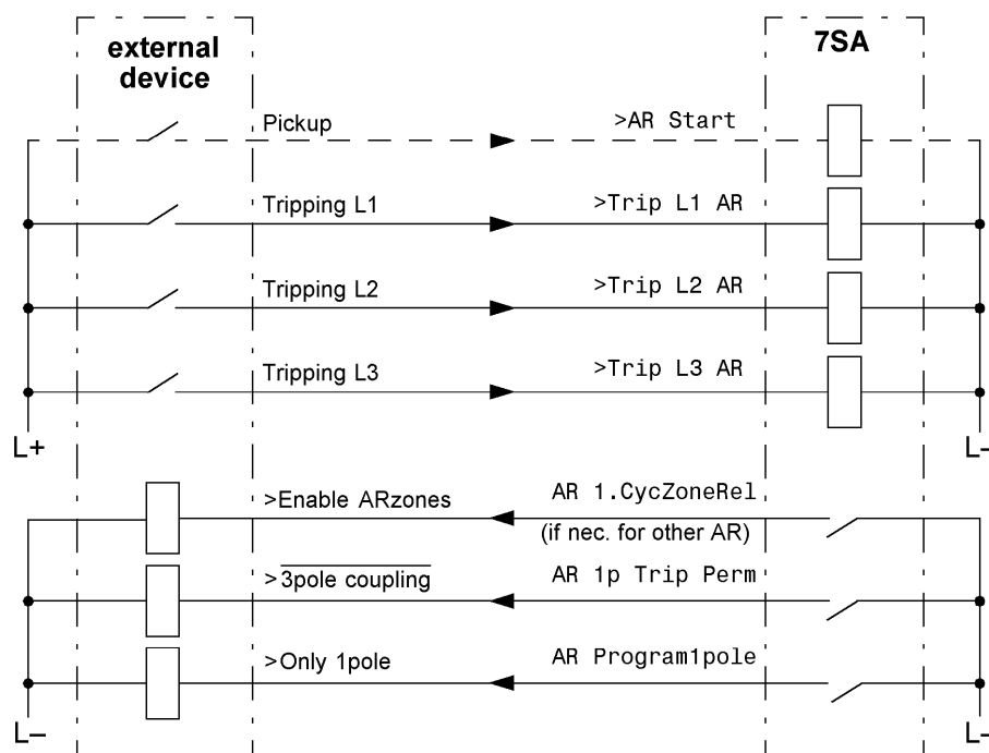
Figure 2-114 Connection example with external protection device for 1-/3-pole reclosure; AR control mode = with TRIP
