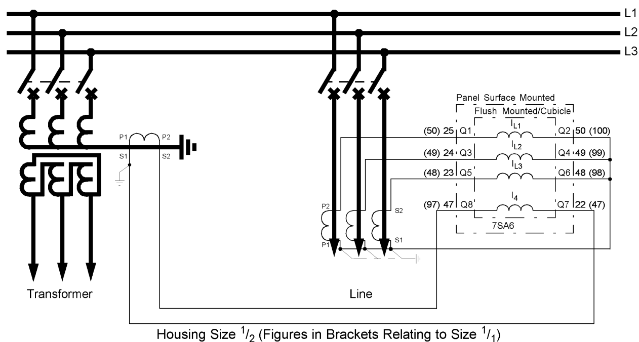
Figure A-38 Current connections to three current transformers and earth current from the star-point current of an earthed power transformer (for directional earth fault protection)
