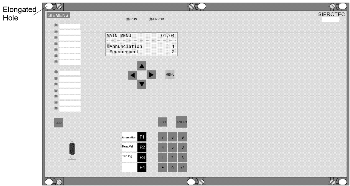
Figure 3-23 Example of panel flush mounting of a unit (housing size \frac{1}{4} )
