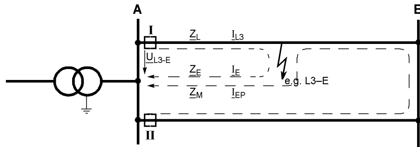
Figure 2-18 Earth fault on a double circuit line
