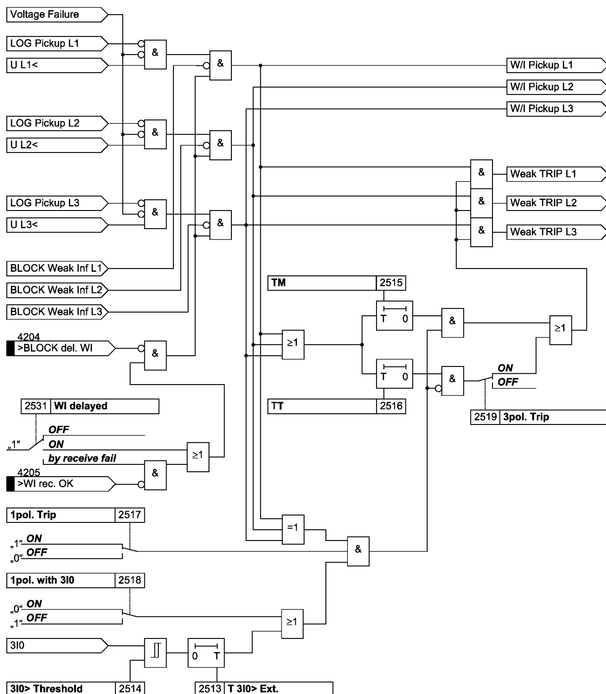
Figure 2-94 Logic for delayed tripping
