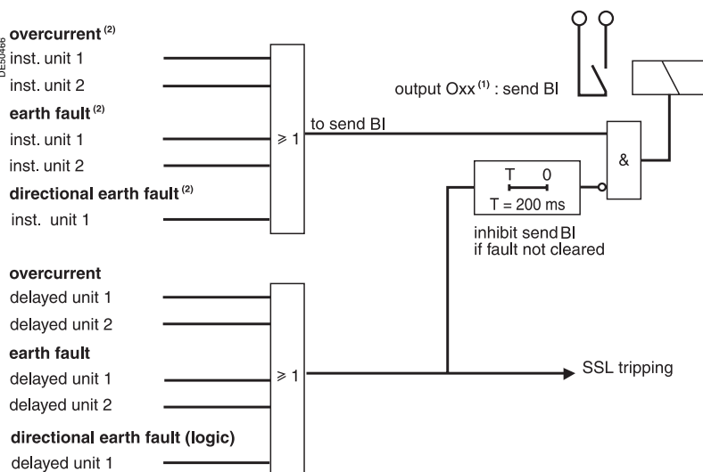
Block diagram: Sepam M41
