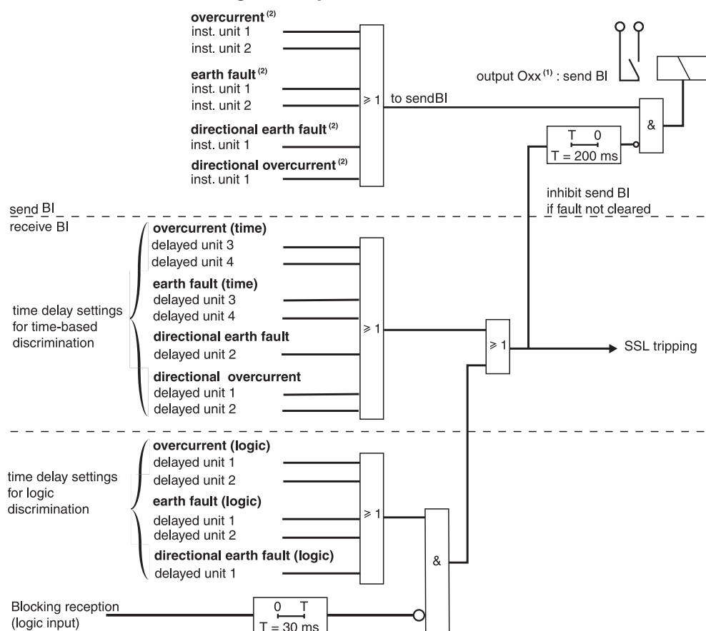
Block diagram: Sepam S40, S41, T40, T42, G40
