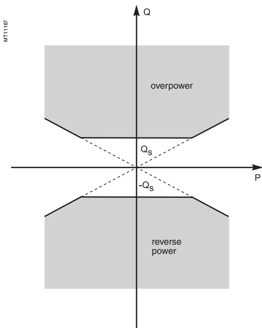
Operating zone.
