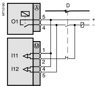
Wiring for shunt trip unit.
