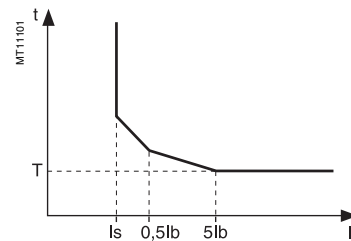
Schneider curve.
