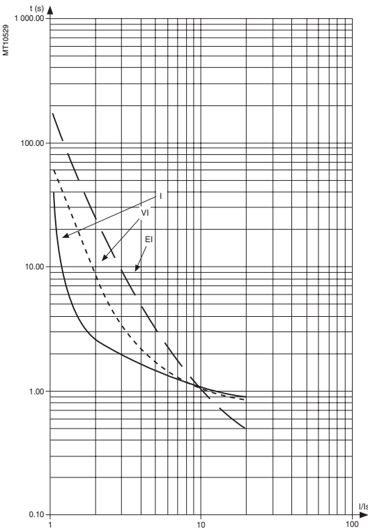
IAC curves
