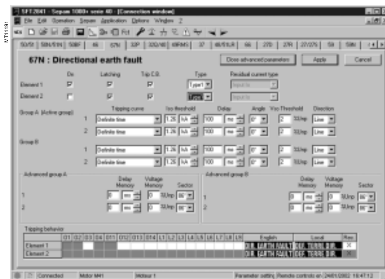
Example of a protection setting screen.
