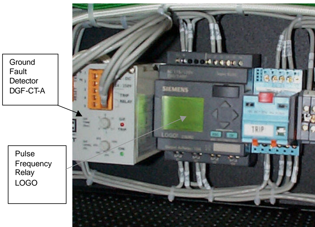
Figure 5 : Control Relays
