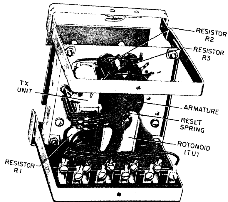
Fig. 2 (8007803) Type RPM21 Relay Removed from Case (Rear View)
