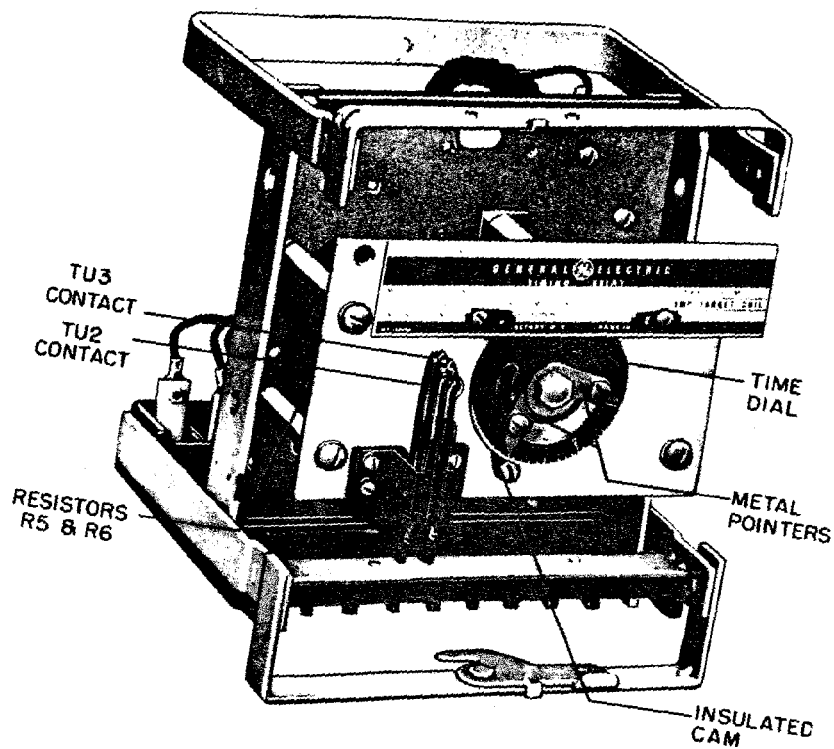
Fig. 1 (8027902) Type RPM Relay Removed from Case (Front View)
