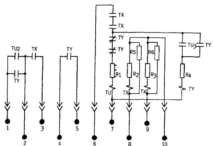
Fig. 7 (0127A9442-3) Internal Connections for RPM24B and RPS24D Relays (Front View)
