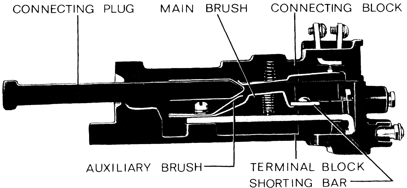
Figure 8 (6077069-4) Barrel Contact Assembly for Ground Fault and Phase Fault Detectors
