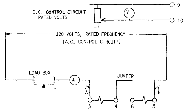
TEST CIRCUIT AS SHOWN IS FOR CHECKING PFD PICK-UP FOR A PHASE-1 TO PHASE-2 FAULT. FOR OTHER PHASE-TO-PHASE FAULT TESTS ON THE PFD AND GFD TEST CONNECTIONS, SEE TABULATION FOR THE RELAY TERMINAL NUMBERS.
