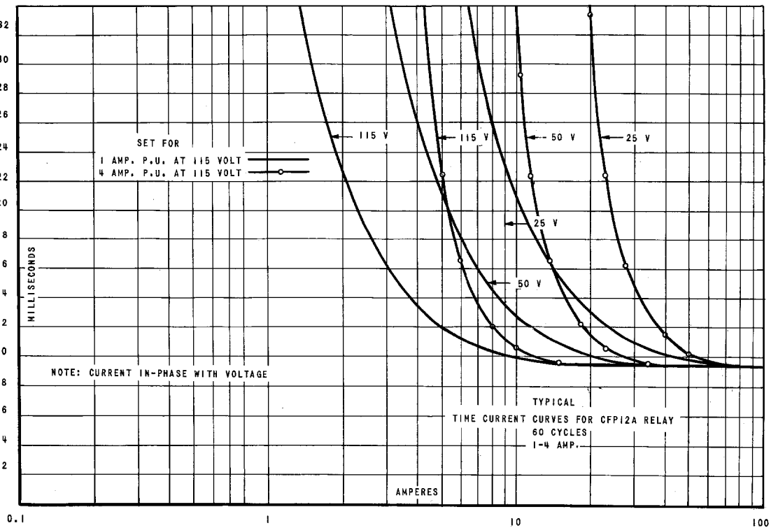
Fig. 4 Typical Time-Current Curves For Type CFPP12A Relays Rated 60 Cycles, 1 To 4 Amperes
