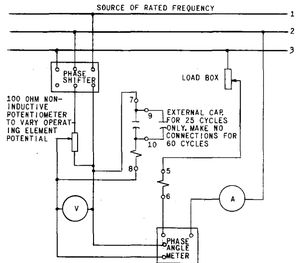
Fig. 9 Test Connections For The Type CFPP11A Relay
