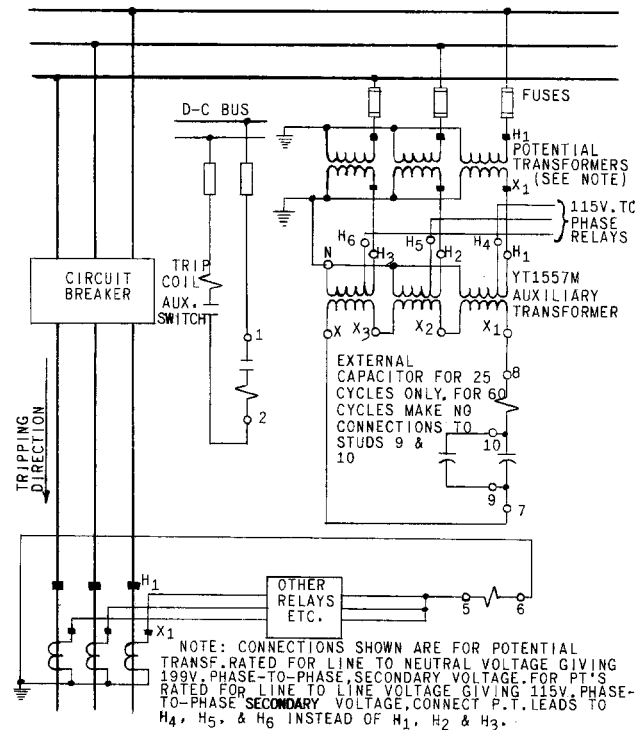
Fig. 10 External Connections For Directional Ground Protection With A Type CFPP1IA Relay
