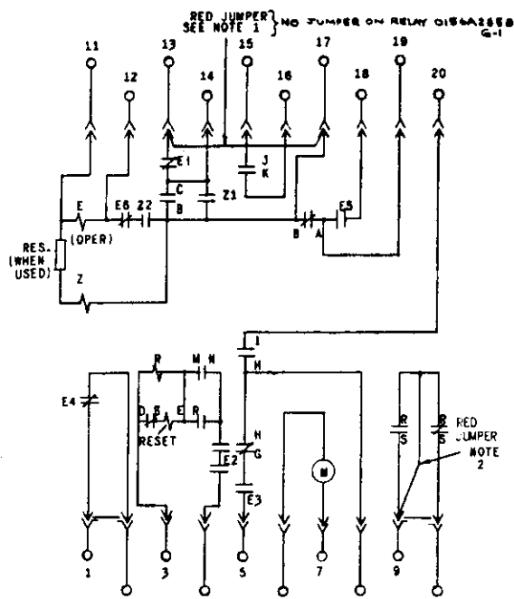
Fig. 2A (362A571-5) Internal Connections for Relay Type ACR11B
