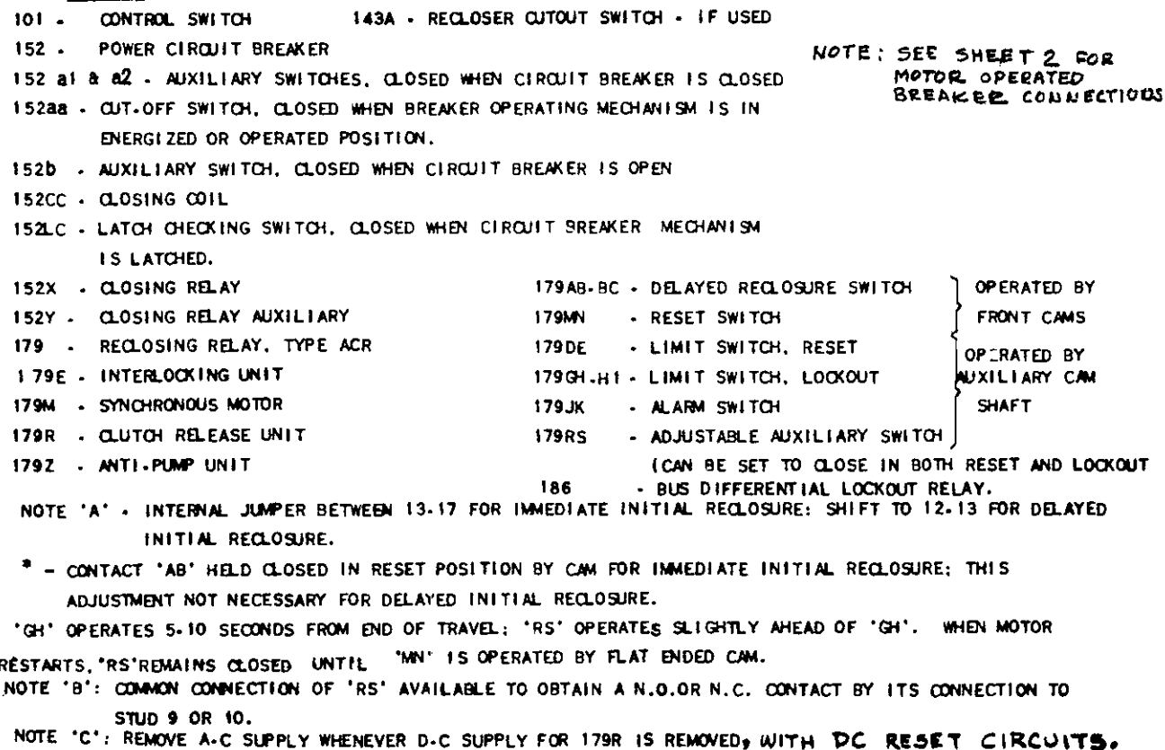
Fig. 3 (362A572-15) Elementary Diagram, Typical Application of Relay Type ACR Used with Solenoid Operated Circuit Breaker
