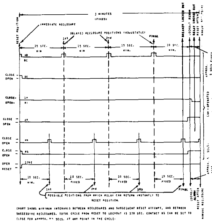
Fig. 6 (362A613-7) Sequence Diagram for Type ACR11B and ACR11E Reclosing Relays
