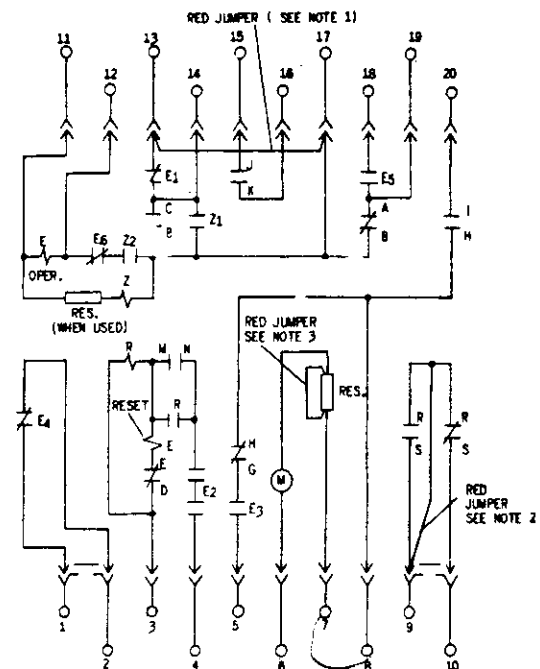
Fig. 2B (104A8965-1) Internal Connections for Relay Type ACR11E
