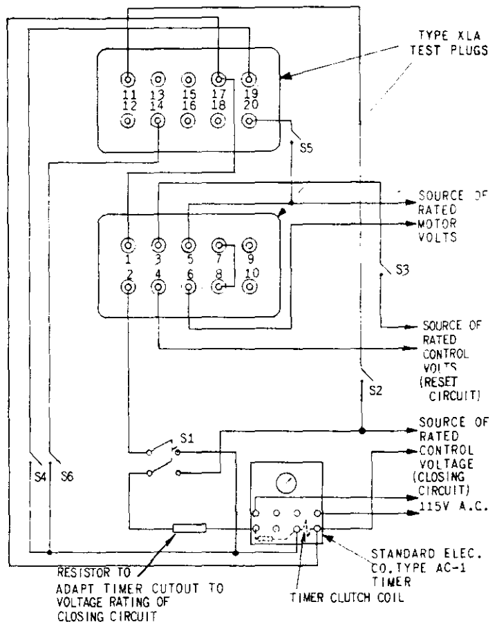
Fig. 9 (362A672-1) Test Connections for Relay Type ACR
