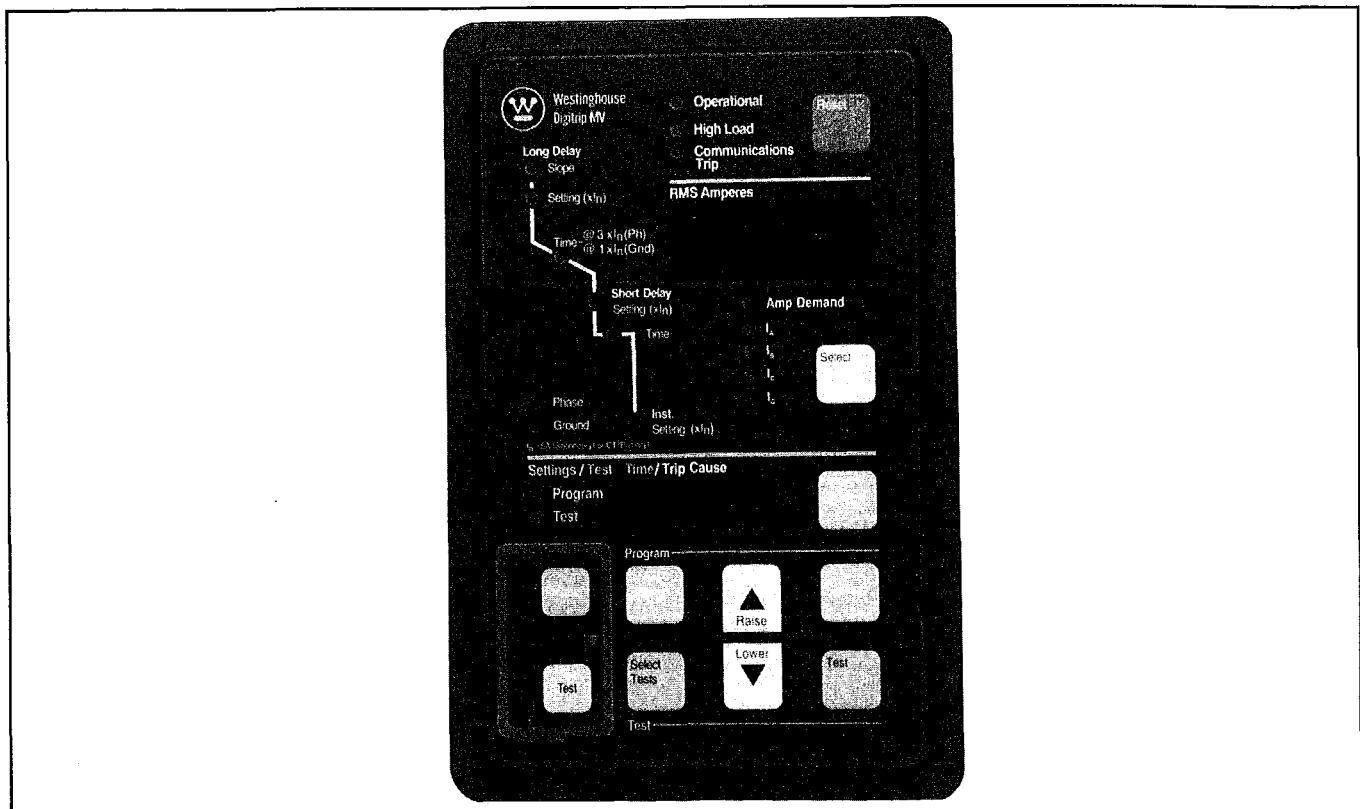
Figure 1-1 Digitrip MV Trip Unit (Front View)
