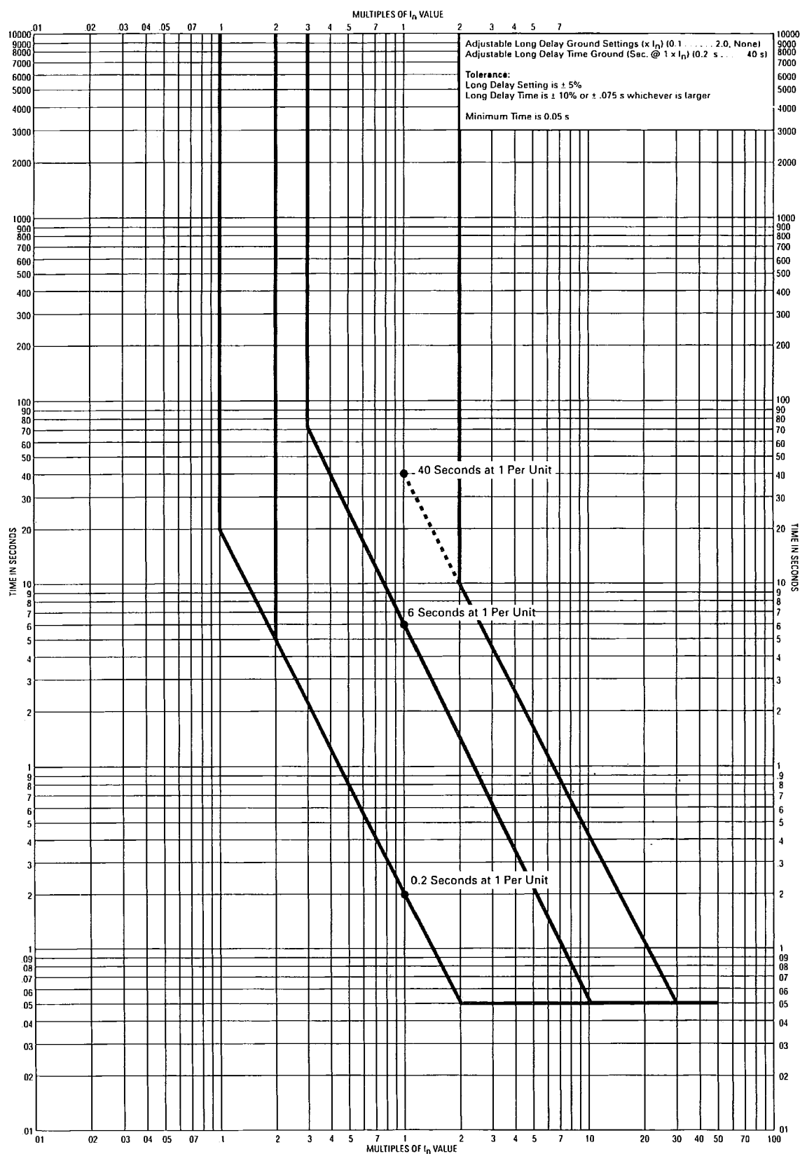
Figure 7-9 Long Delay Ground, I^2T Curves (SC-5400-92).
