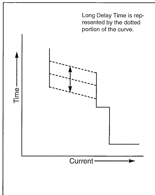
Figure 3-6 Typical Phase Long Delay Time Adjustment (IT Response).
