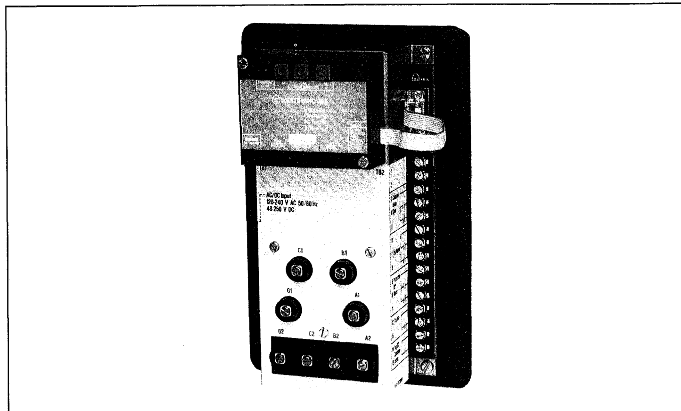
Figure 1-2 Digitrip MV Trip Unit With Installed INCOM PONI Module (Rear View).
