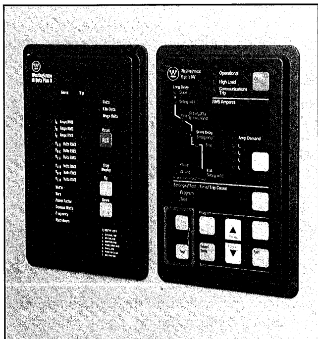
Figure 1-3 A Digitrip MV Trip Unit [RHS] Installed on a Metal Assembly Panel.
