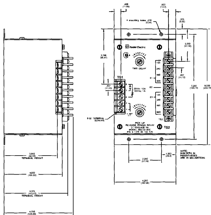
FIGURE 5. BE3-32-3 OUTLINE DRAWING
