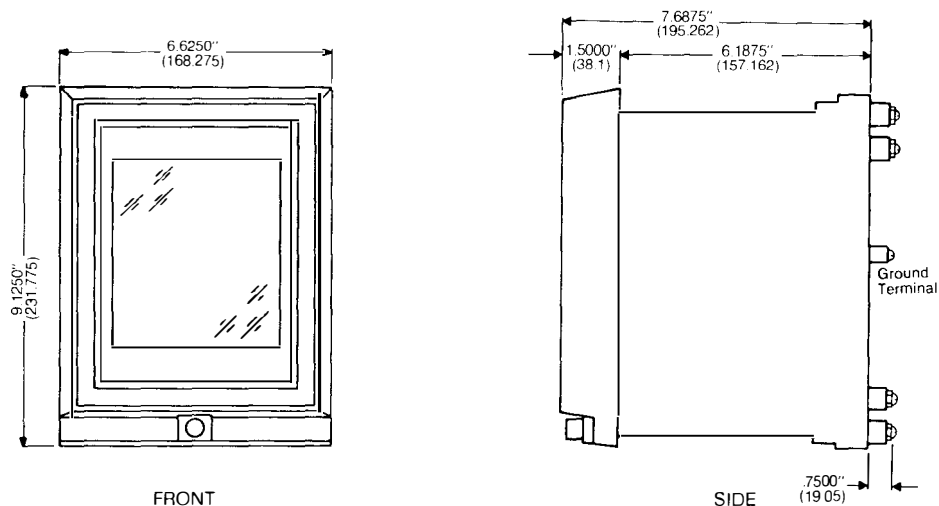
FIGURE 6. OUTLINE DRAWING
