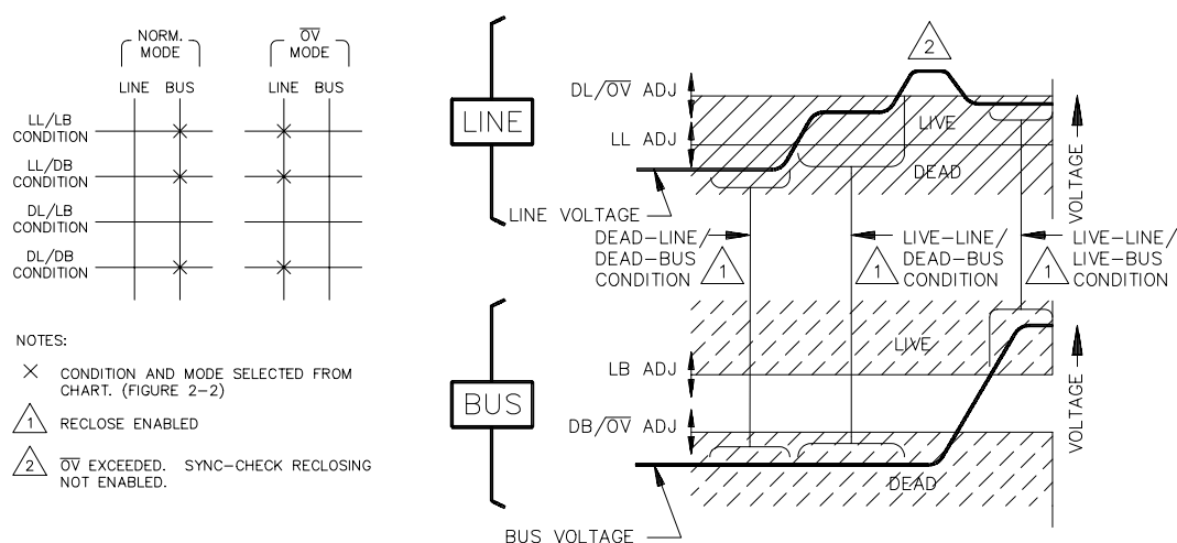
SELECTED LIVE-LINE/LIVE-BUS, LIVE-LINE/DEAD-BUS AND DEAD-LINE/DEAD-BUS CONDITIONS, WITH OV FOR THE LIVE-LINE
