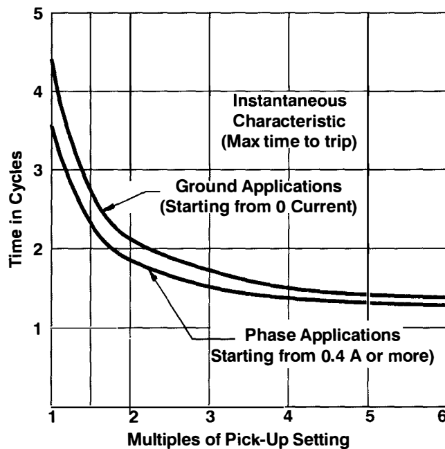
Figure 3 - Instantaneous Characteristics
