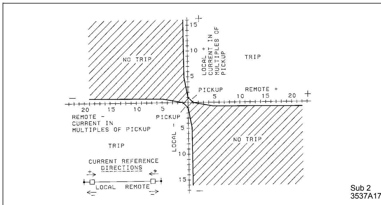
Figure 18: LCB Operating Characteristics (IN/OUT phase)
