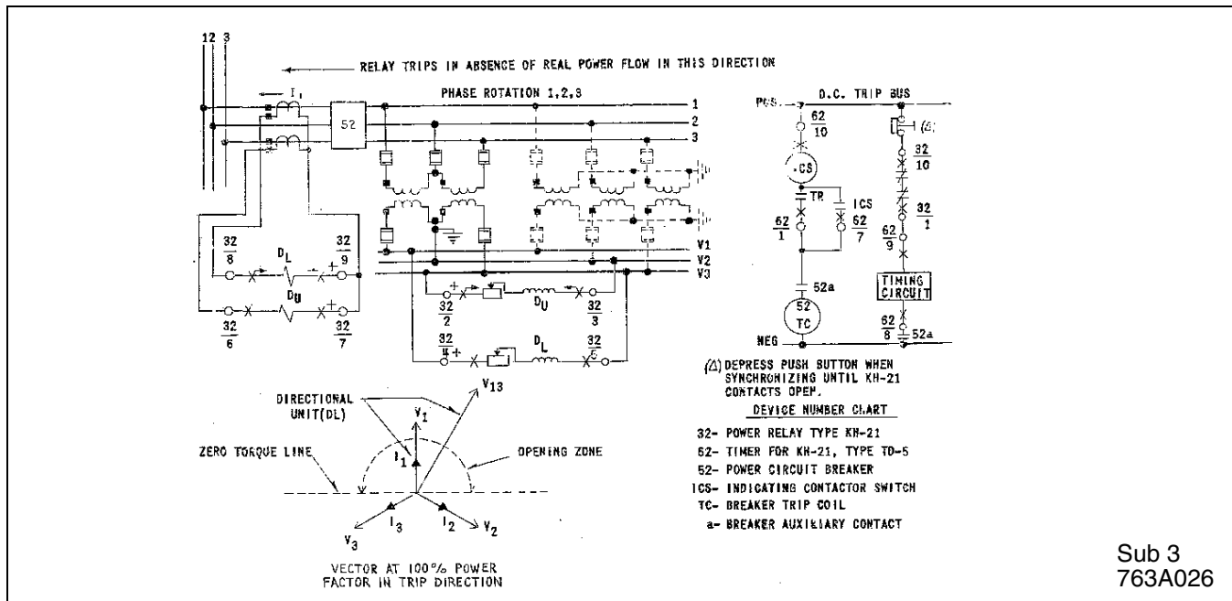
Figure 3. External Schematic
