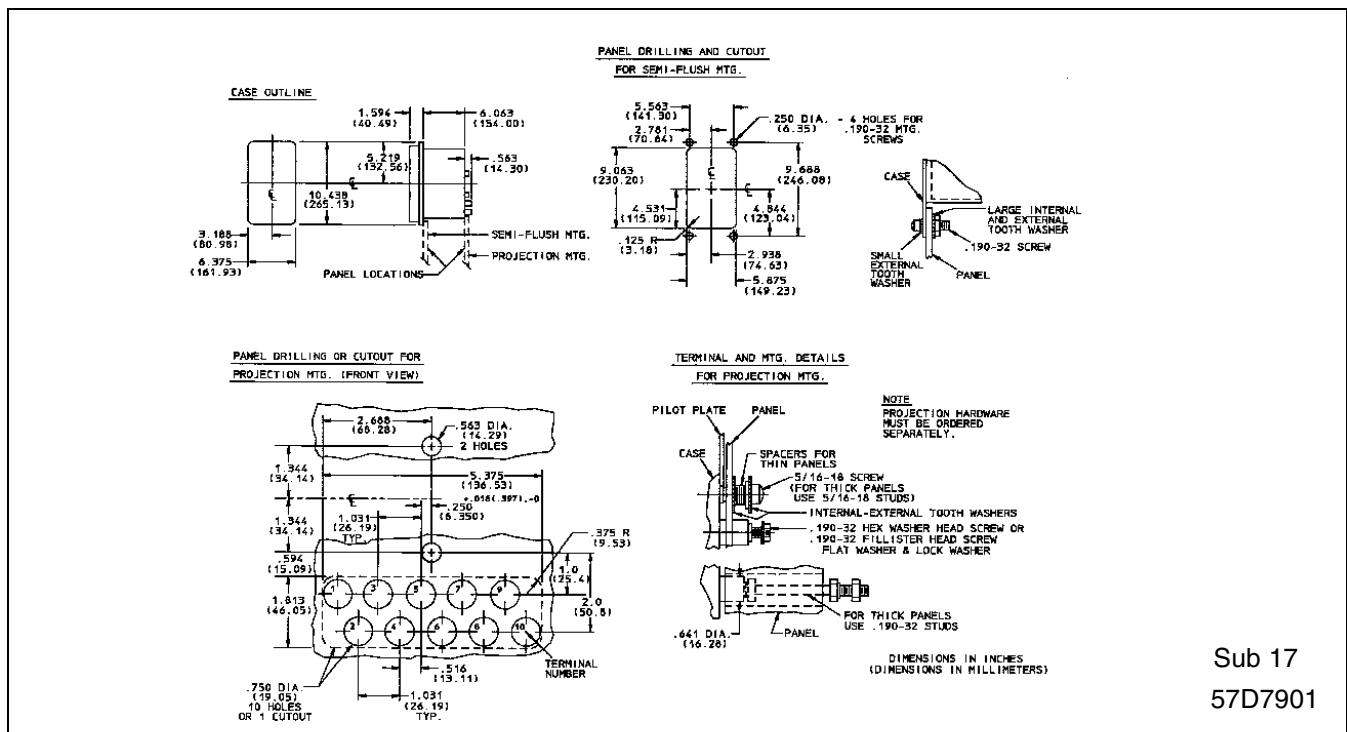
Figure 2. Outline and Drilling (Type FT-21 Case)
