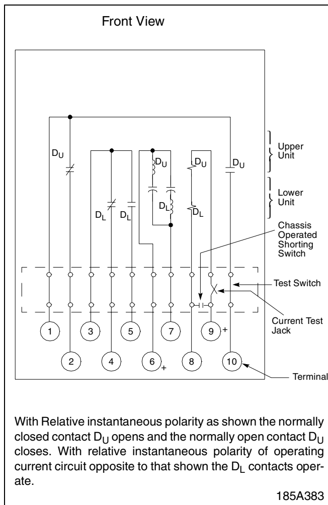
Figure 1. Internal Schematic (Without IT Unit).
