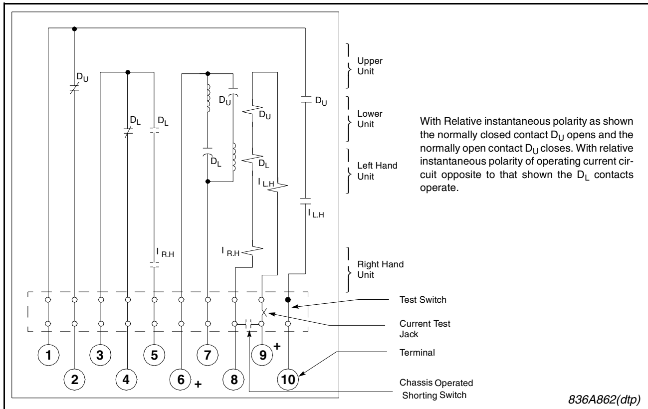
Figure 2a. Internal Schematic (with IT Units) (.5 to 2 amp range)
