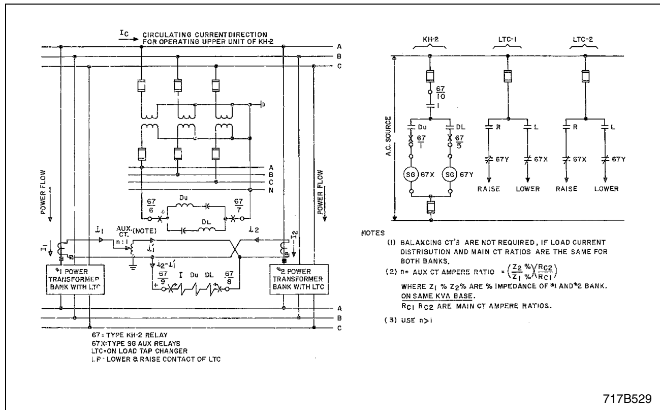
Figure 3. External Schematic
