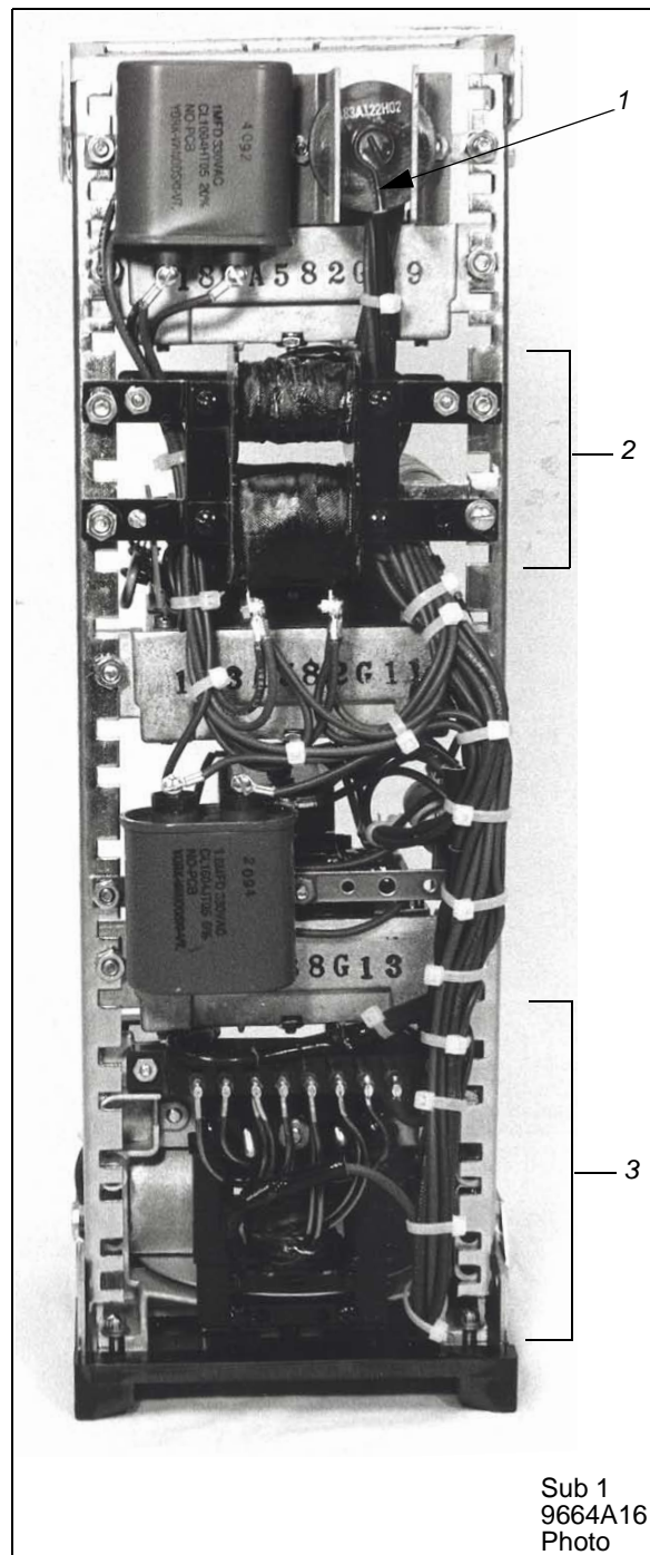
Figure 2: Type IRD Relay without Case (Rear View)
