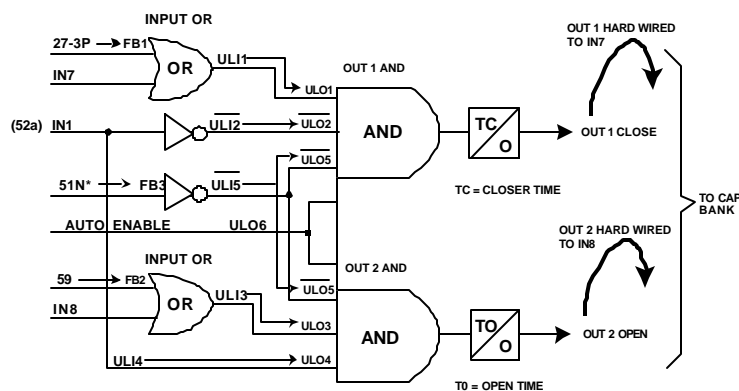
Figure 1 - Capacitor Bank Control Logic Control
