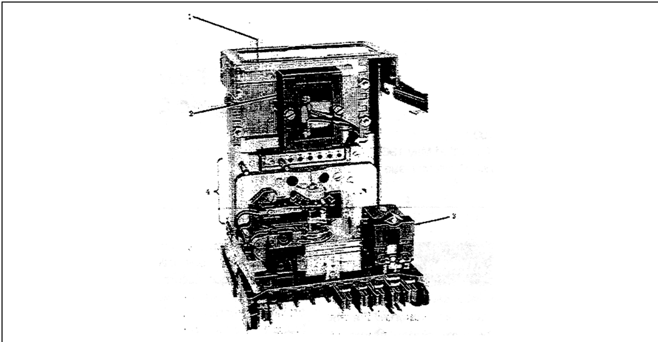
Figure 1. Type CW Relay Without Case. (1) Capacitor. (2) Reactor. (3) Indicating Contactor Switch (ICS). (4) Time-Power Unit.
