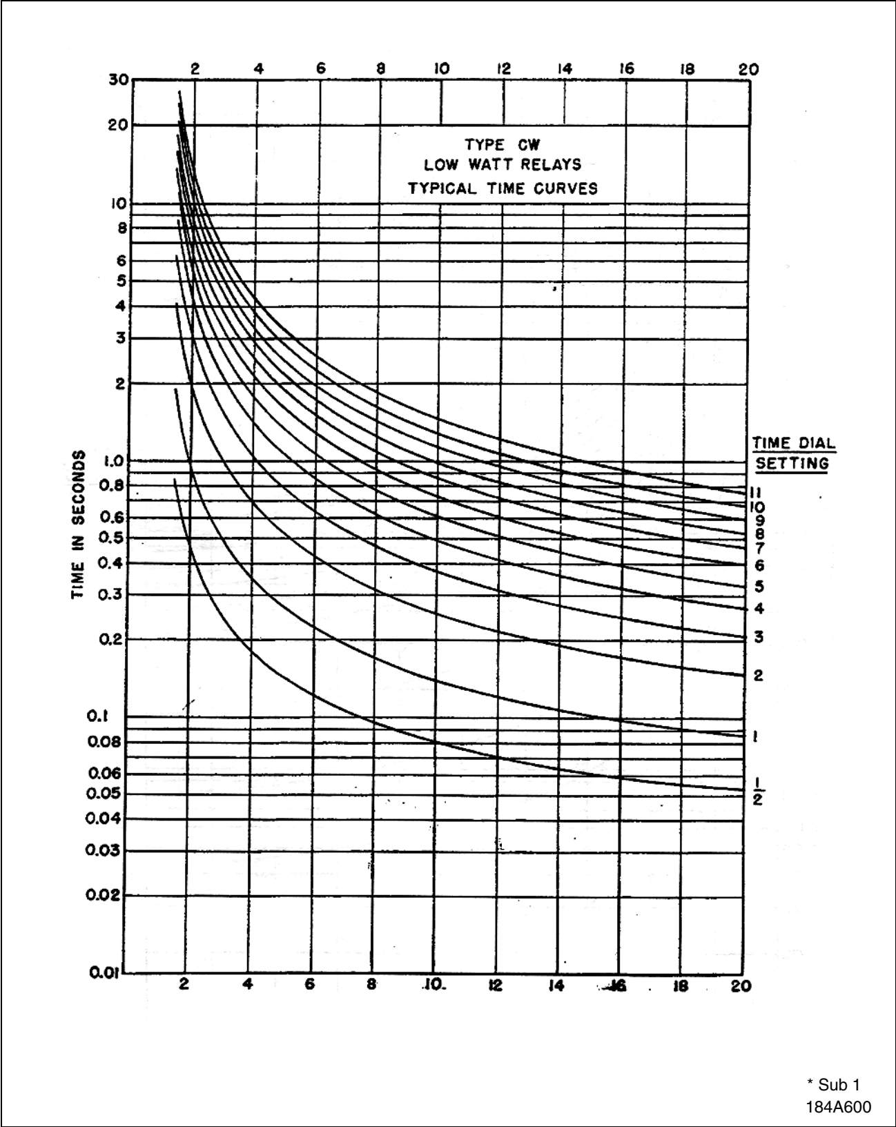
Figure 4. Typical 60 Hertz Time Curves of the 20-120 Watt Type CW Relay.
