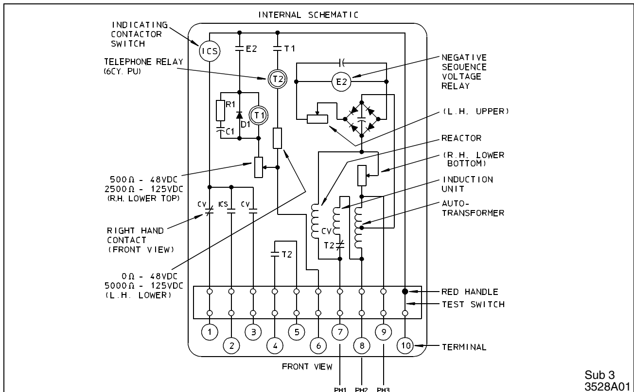
Figure 2: Relay Type CVQ Negative Sequence and Over and Undervoltage Relay with Telephone Relay in FT-31 Case
