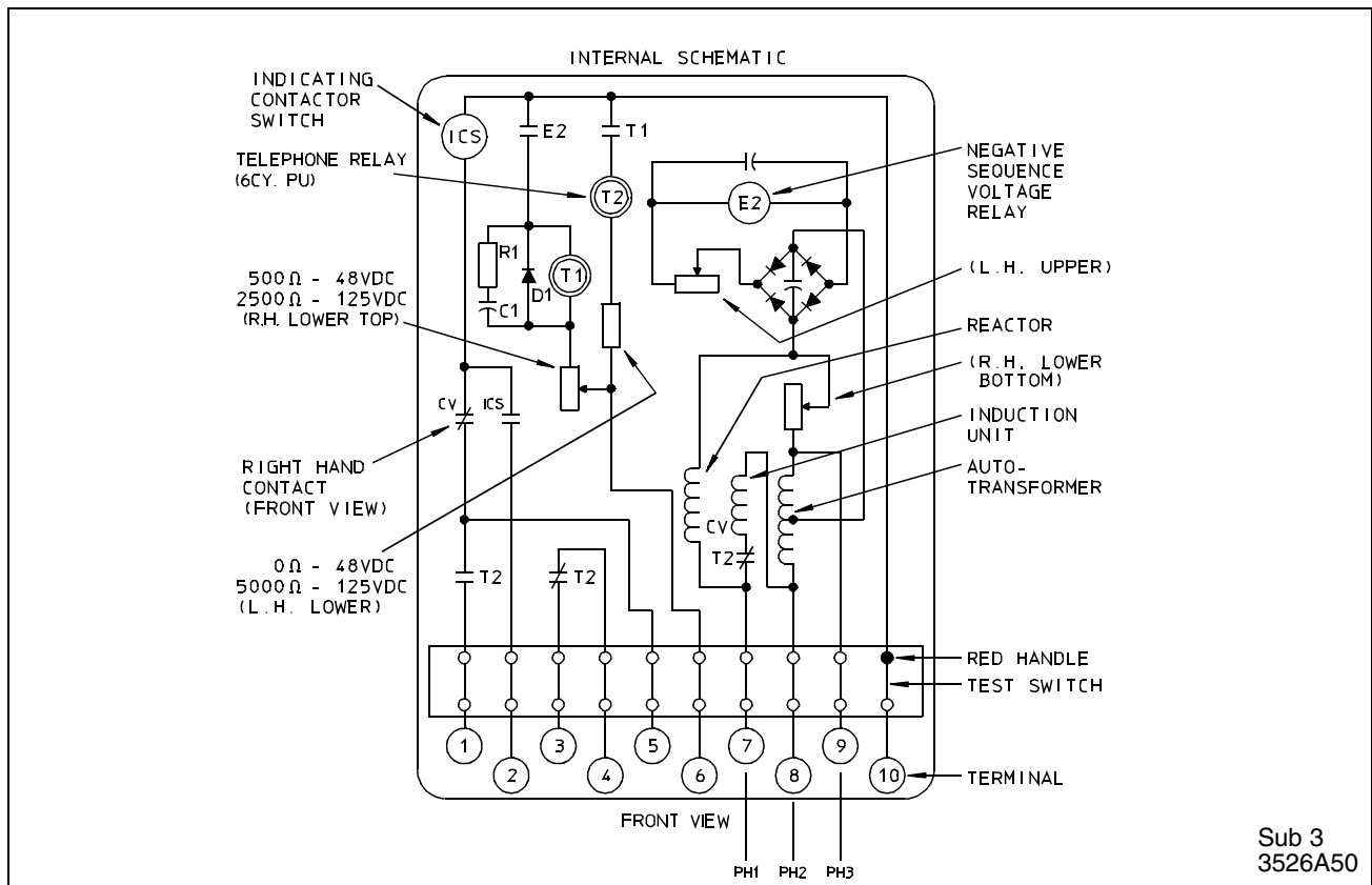
Figure 1: Relay Type CVQ Negative Sequence and Undervoltage Relay with Telephone Relay in FT-31 Case
