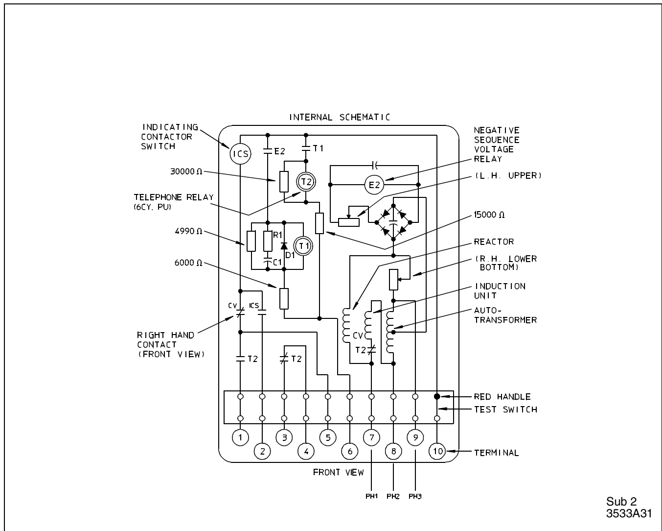
Figure 3: Relay Type CVQ Negative Sequence and Undervoltage Relay with Telephone Relay in FT-31 Case (330 Vdc/Trip Ckt)
