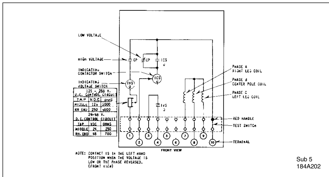
Fig. 2. Internal Schematic of the Type CP Relay with Independent Contacts in the Type FT-11 Case.
