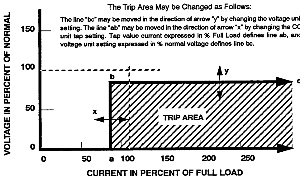
Figure 3. Typical Tripping Characteristics of Type COV Relay
