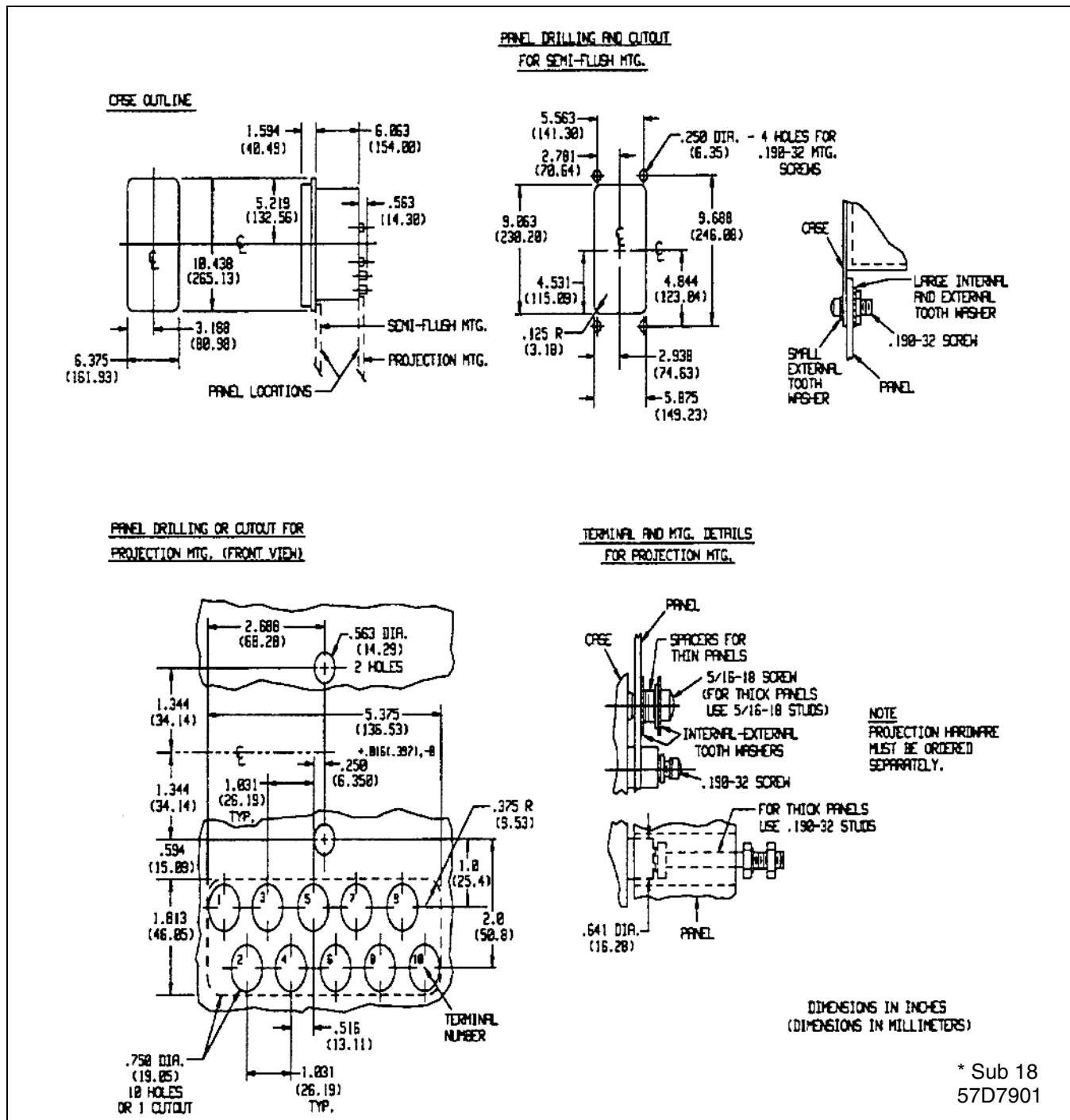
Figure 11. Outline and Drilling Plan for the COQ Relay in the FT 21 Case
