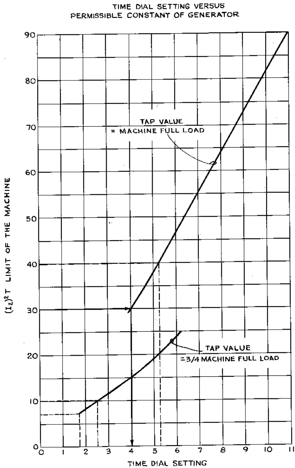
Figure 5. Required COQ Time Dial Setting versus Generator Constant.
