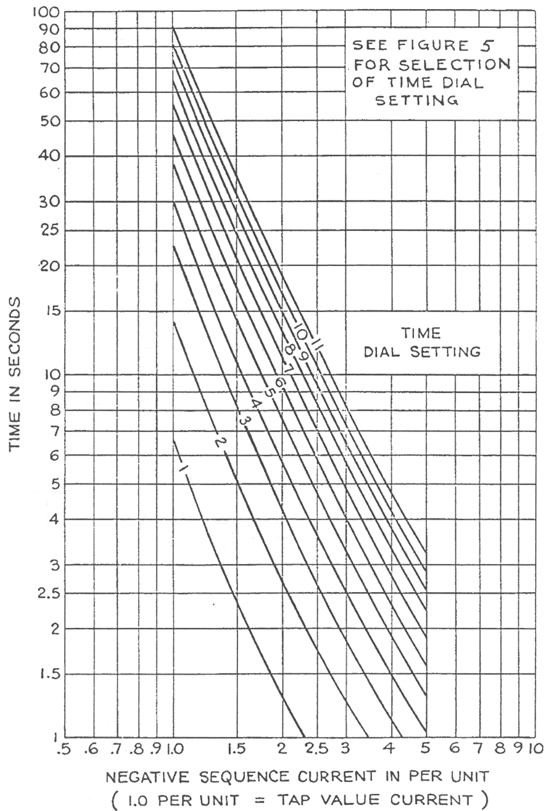
Figure 3. Relay Time - Current Curve.
