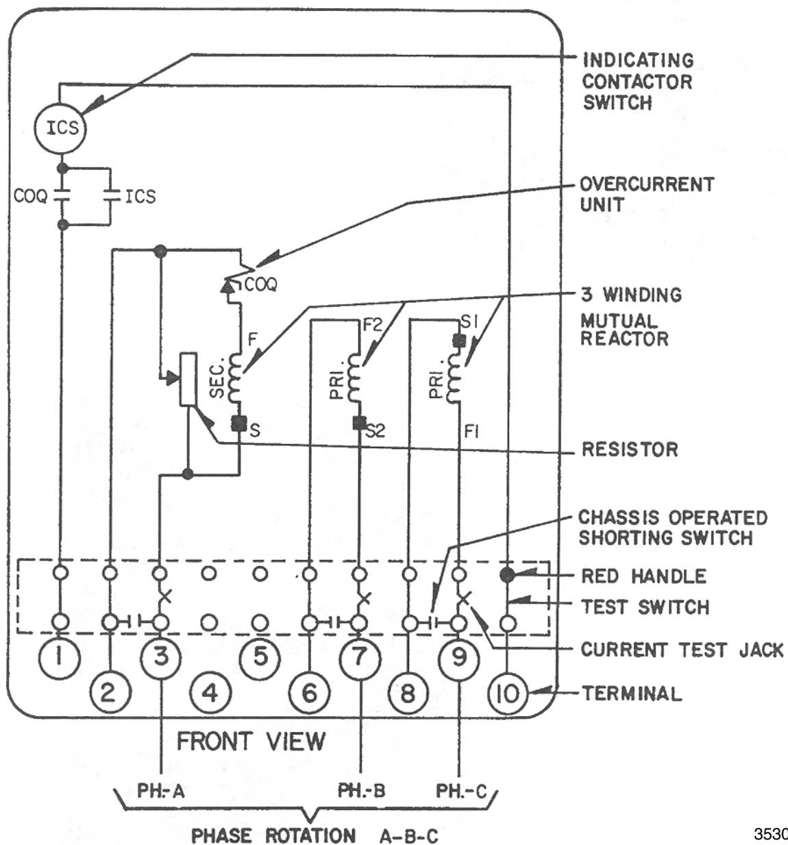
Figure 2. Internal Schematic of the COQ Relay in the FT-21 Case.
