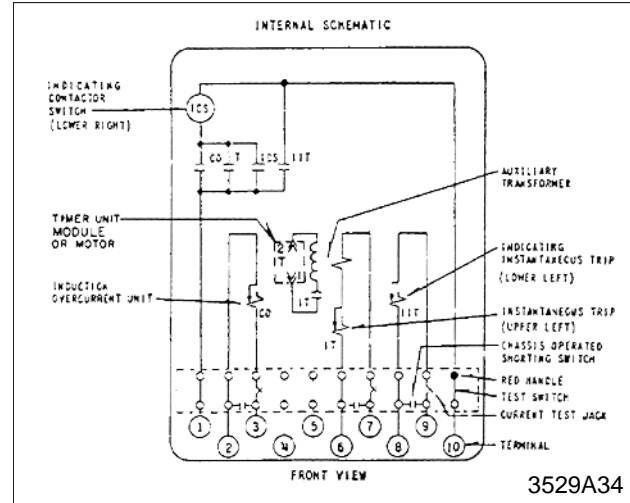
Figure 1: Internal Schematic of the Type CO-4 Relay in Type FT-21 Case.
