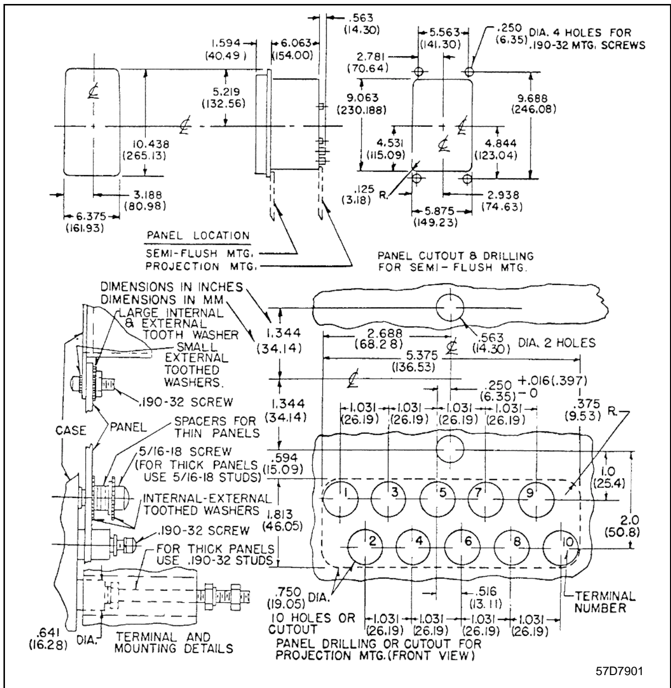
Figure 6 Outline and Drilling for the Type CO-4 Relay in Type FT-21 Case.
