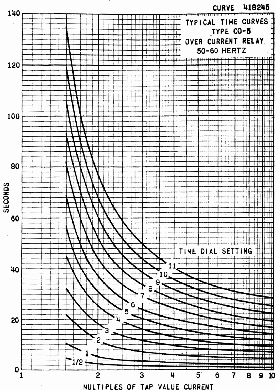
Figure 2: Typical Time Curves for the Overcurrent Unit.
