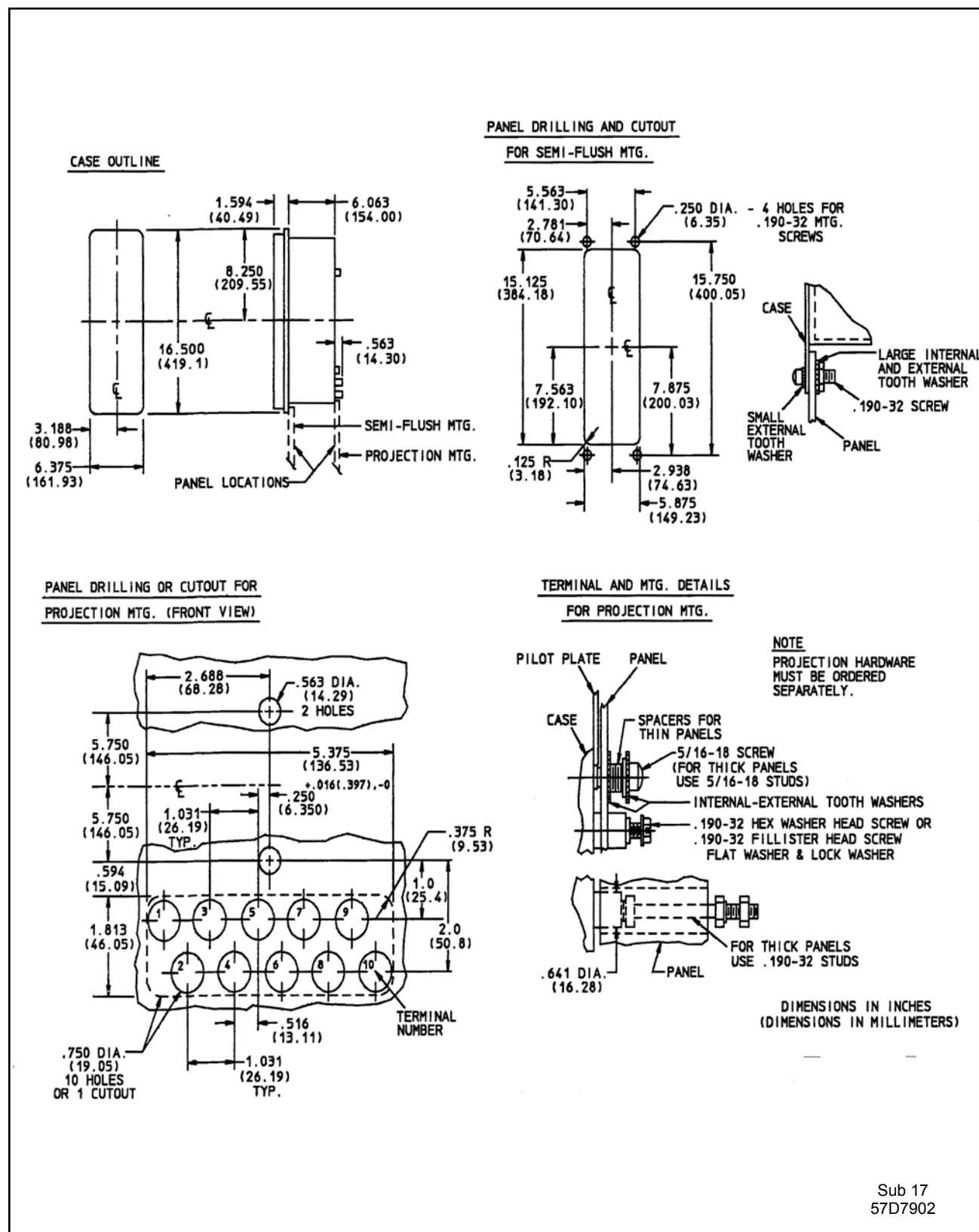
Figure 10 - Outline and Drilling Plan for the Type CM Relay in FT-31 Case
