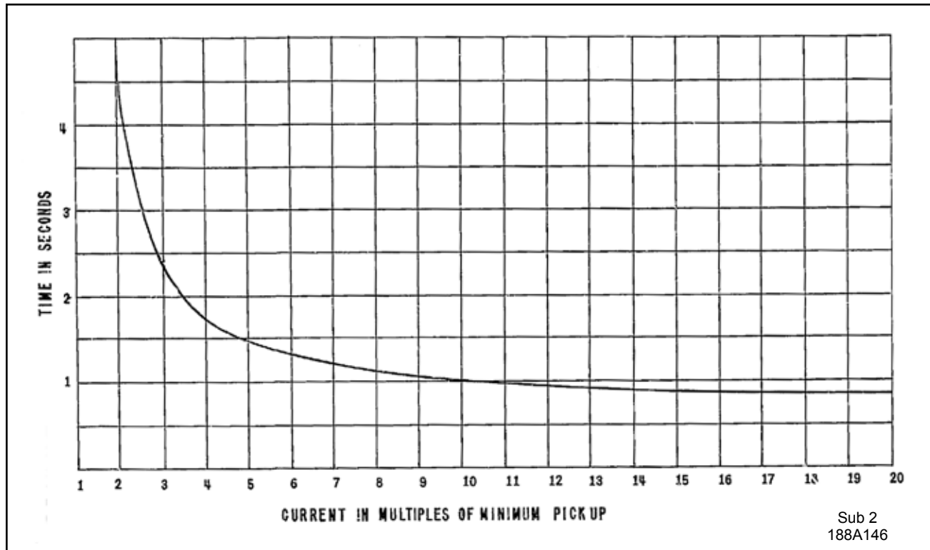
Figure 4 - Typical Time Curve with Zero Restraint of the Type CM Relay
