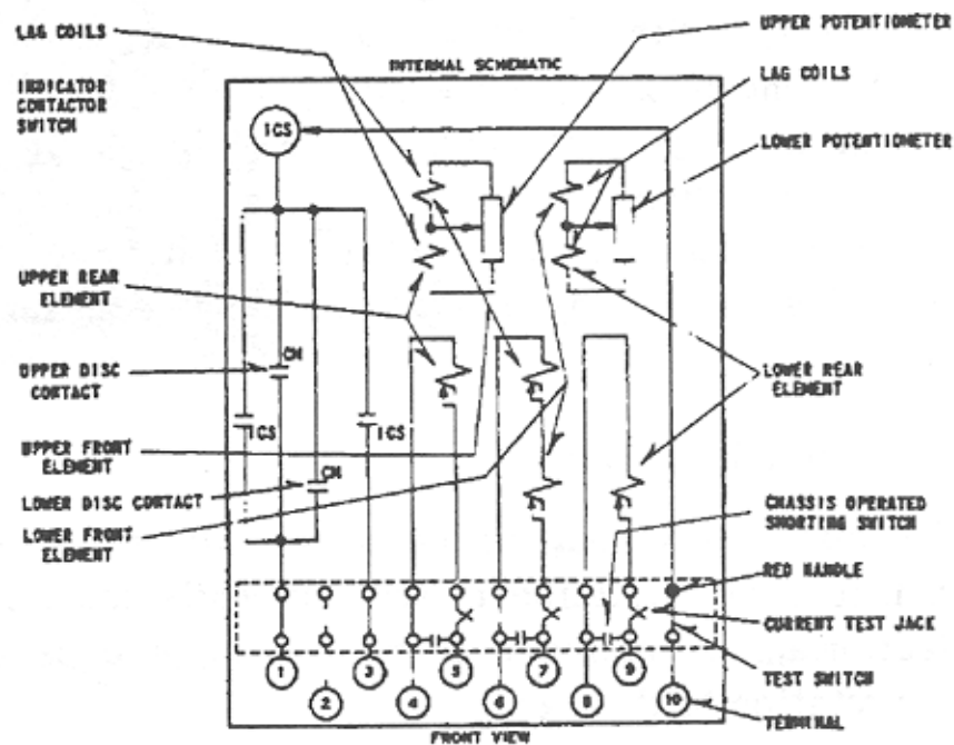
Figure 8. Internal Schematic of the Tapped Type CM Relay in the Type FT-31 Case
