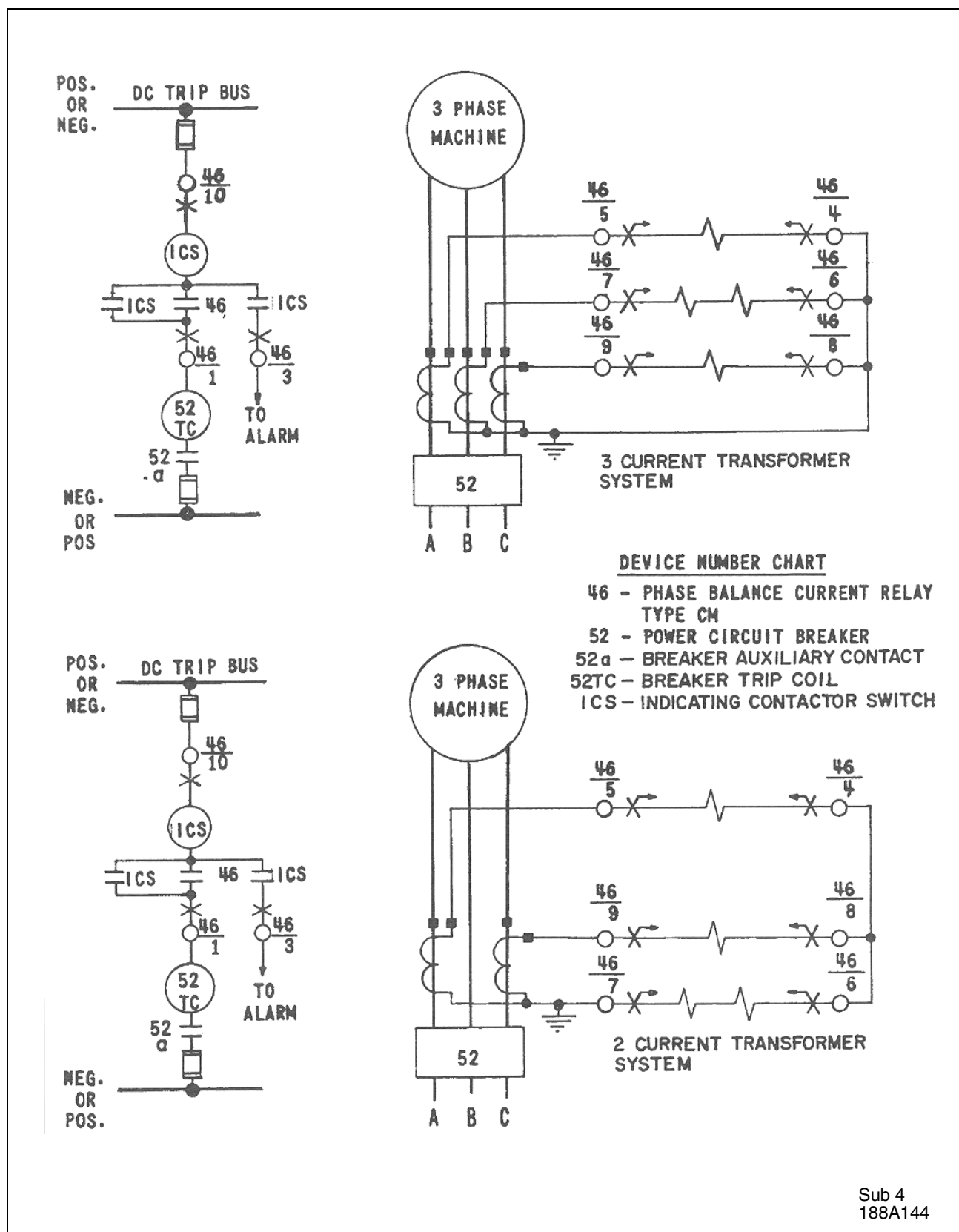
Figure 10. External Schematic Diagram of the Type CM Relay in the Type FT-31 Case
