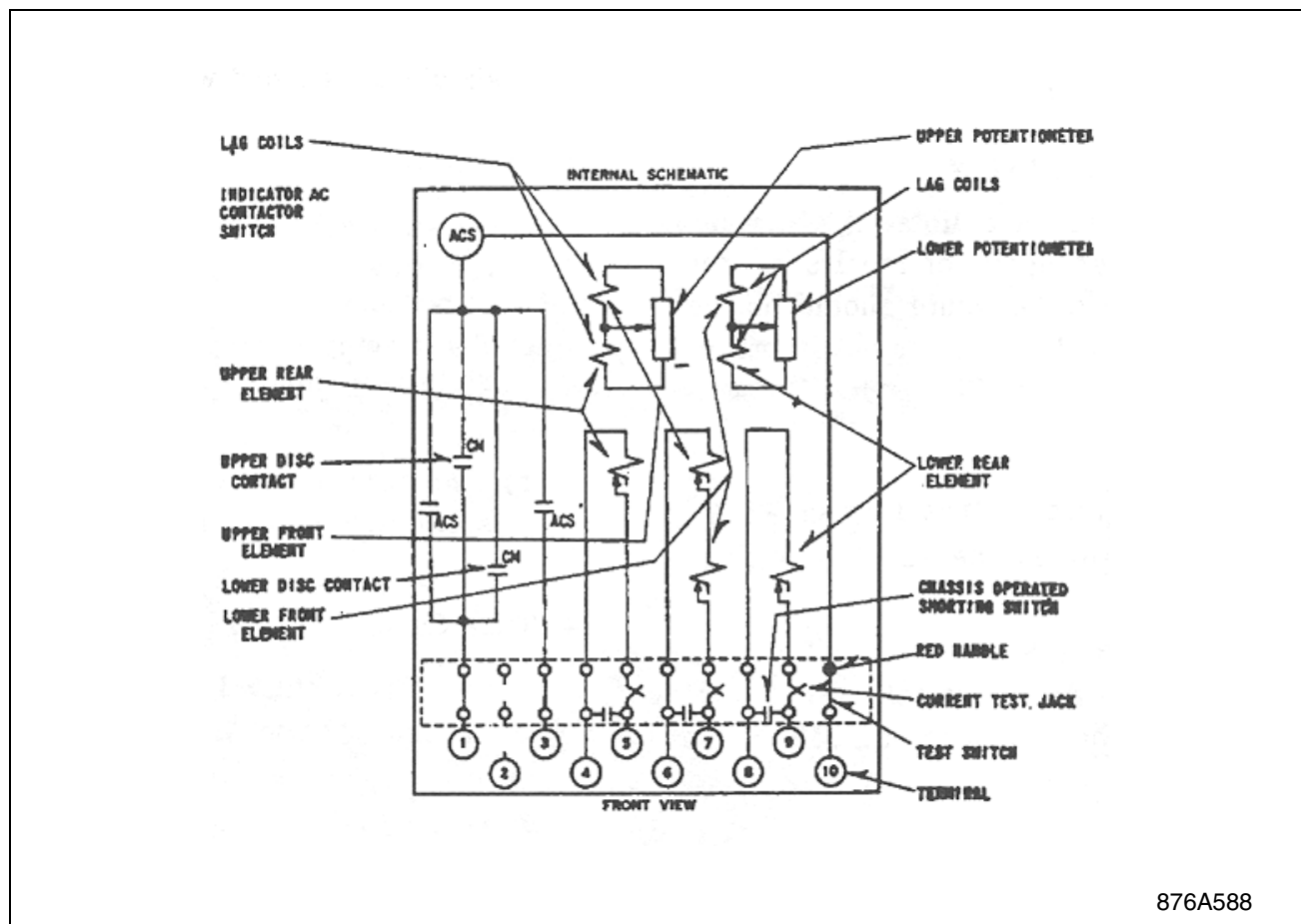
Figure 6. Relay Type CM Phase Balance Current With Taps And Acs Unit In Type FT-31 Case.
