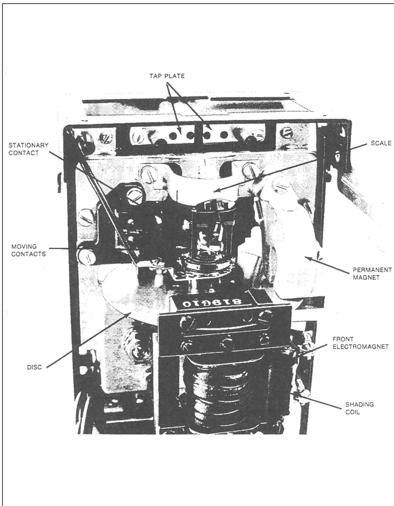
Figure 9. Element Assembly for CM Relay (Front View)
