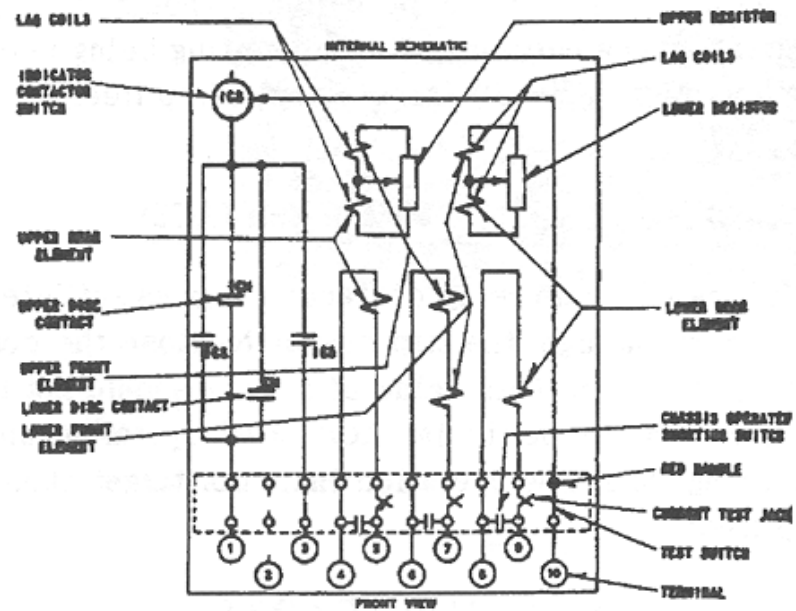
Figure 7. Internal Schematic of the Non-Tapped Type CM Relay in the Type FT-31 Case
