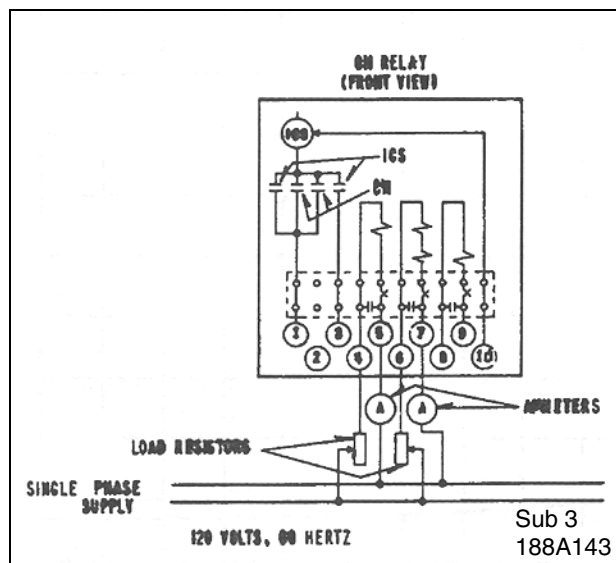
Figure 5. Diagram of test connection for the non-tapped Type CM Relay in the FT-31 Case. For tapped CM place tap screw in 1 amp. tap setting.
