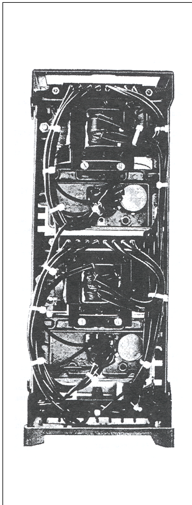
Figure 2b. Type CM Tapped Relay without case (Rear View)
