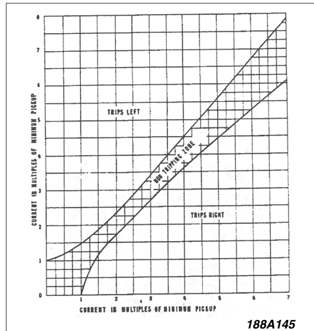
Figure 3. Typical Operating Curve of the Type CM Relay
