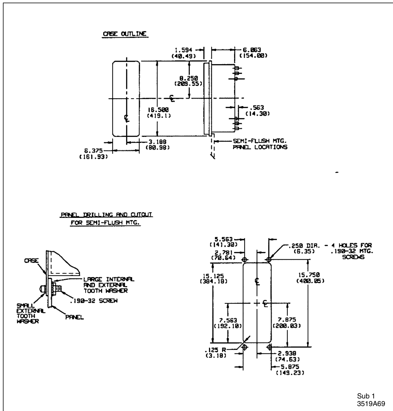
Figure 11. Outline and Drilling for the CA-16 Relay in FT-32 Case
