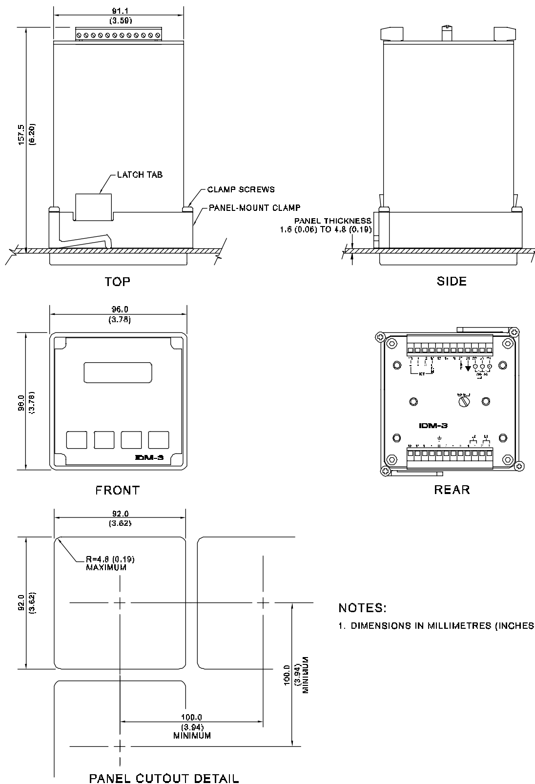
PANEL-MOUNT IDM-3 OUTLINE AND MOUNTING DETAILS
