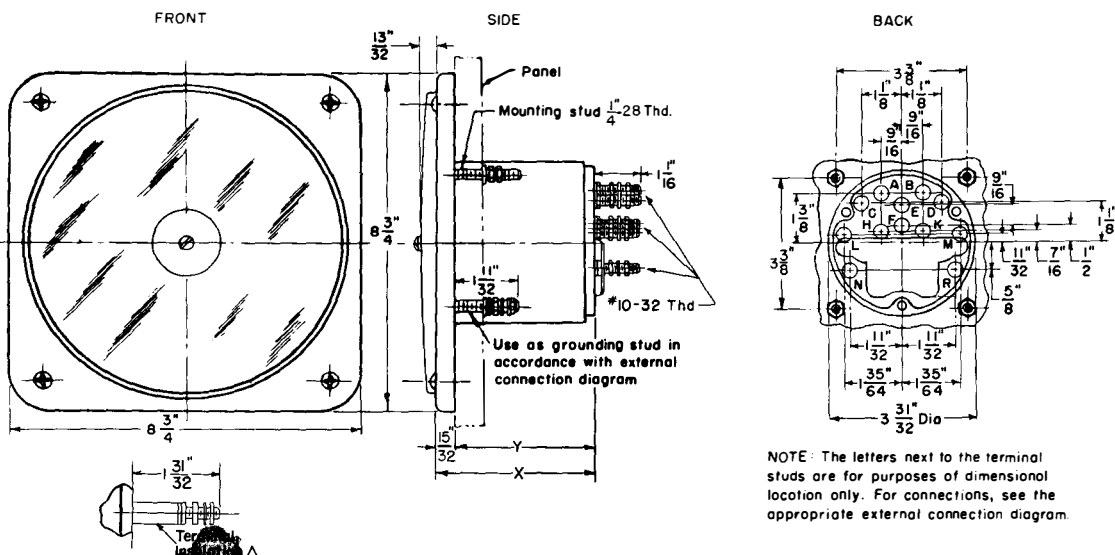
Fig. 1. Dimensions of Types AB-14,-15, and -19 wattmeters.
