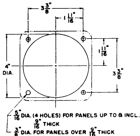
Fig. 1. Cut-out and panel drilling dimensions
