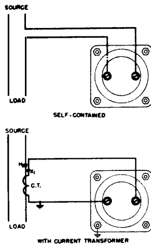
Fig. 5. External connections of a-c ammeter
