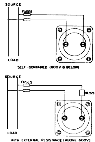
Fig. 7. External connections of a-c voltmeter
