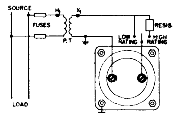
Fig. 10. External connections of double-rated a-c voltmeter with potential transformer
