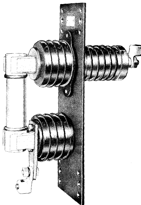
Fig. 6 EK-1C with One Front Connected and One Back Connected Insulator
