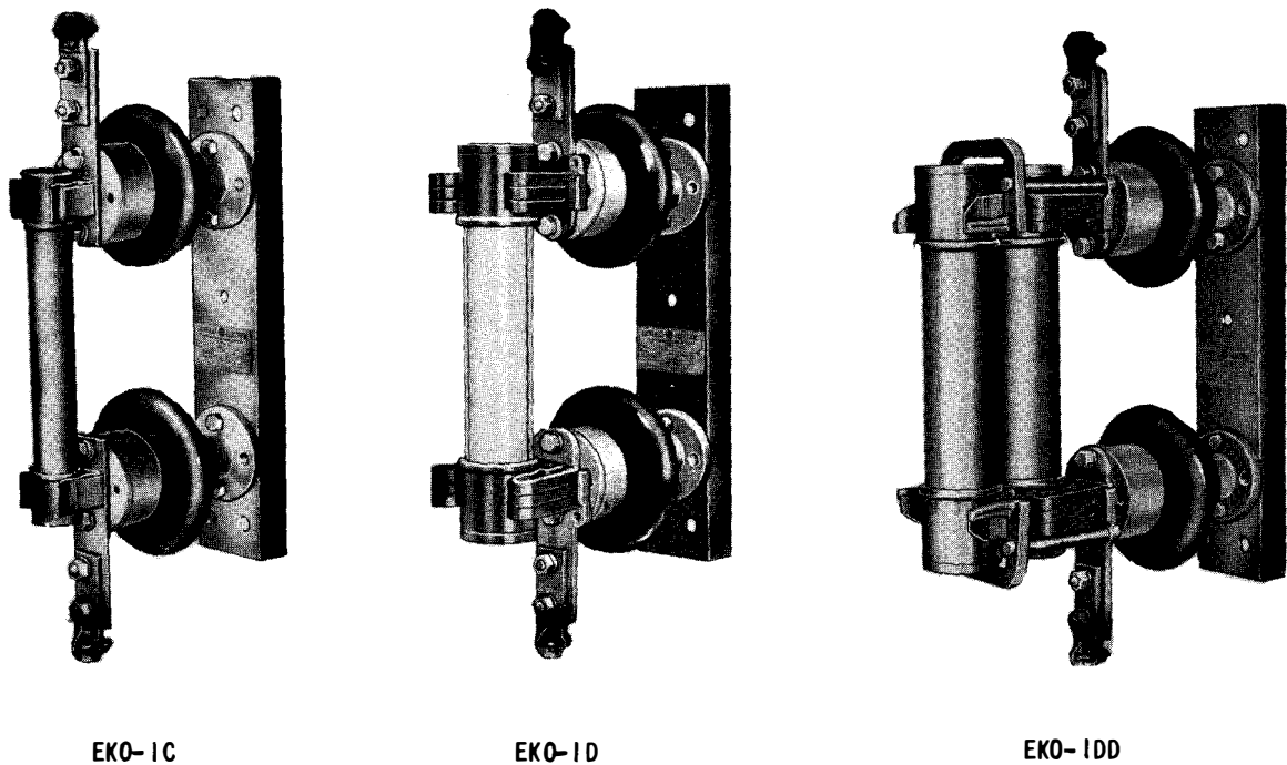
Fig. 3 Type EKO-1 Fuse Supports
