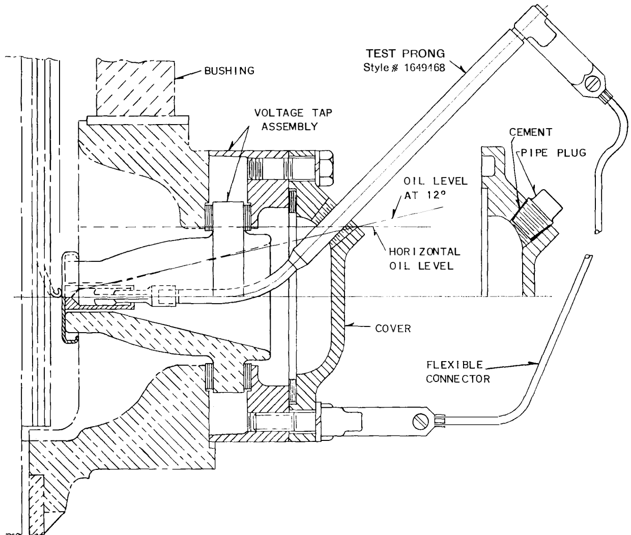
TEST PRONG FOR MAKING UNGROUNDED P.F. TESTS THROUGH VOLTAGE TAP ON TYPE "O" BUSHINGS
