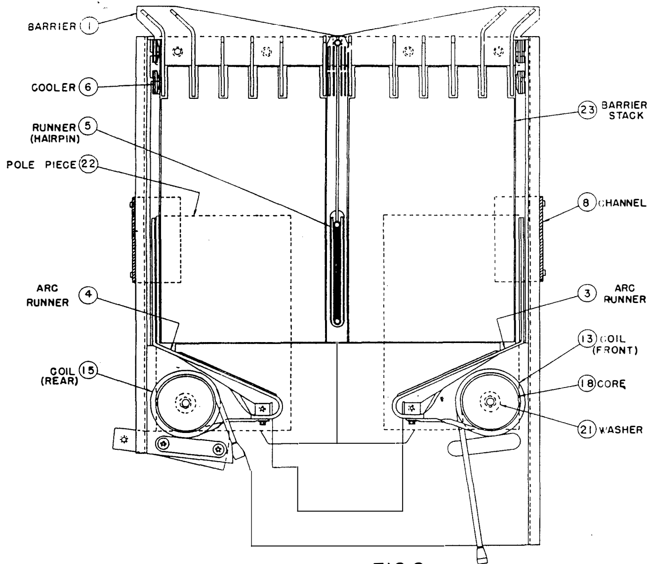
FIG.2 TYPICAL ARC CHUTE
