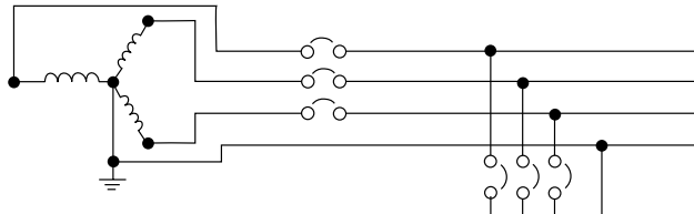
Figure 5. Four-Wire Distribution, Solidly Grounded System
