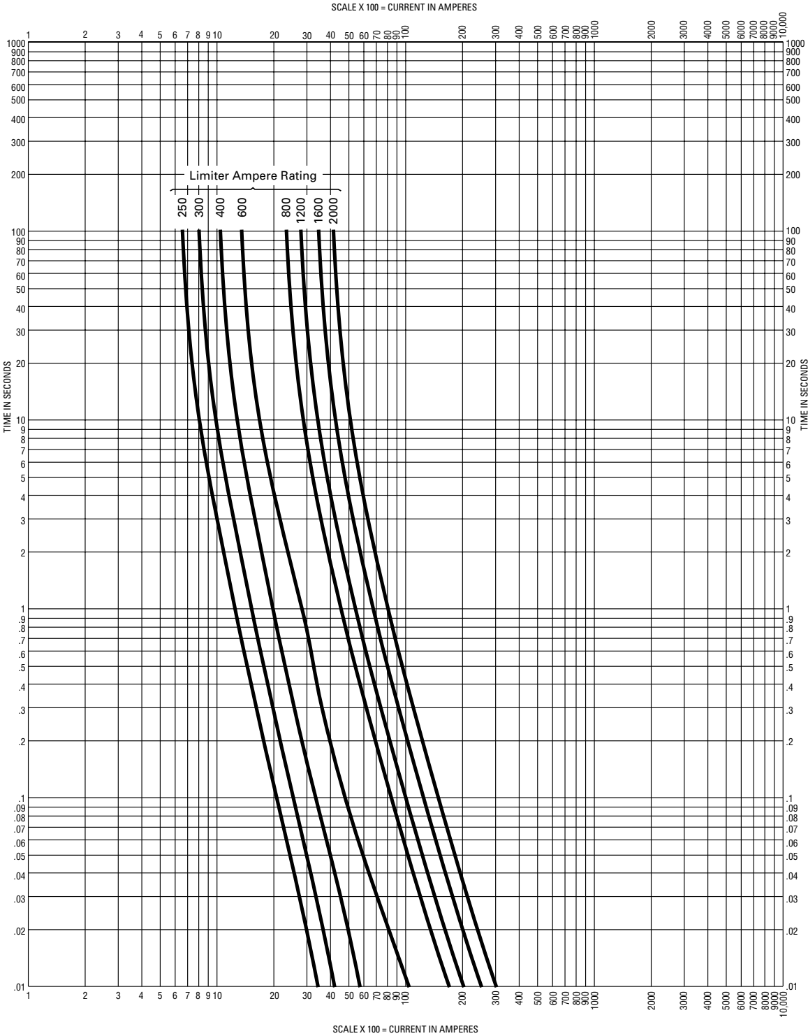
DSLII-308 Average Melting Time-Current Characteristics
