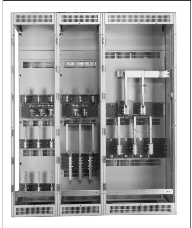
Cable Connection Compartment with Barriers in Place
