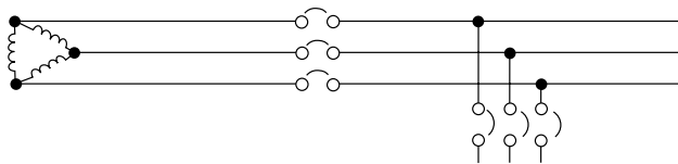
Figure 1. Three-Wire Distribution, Delta Source (Ungrounded)
