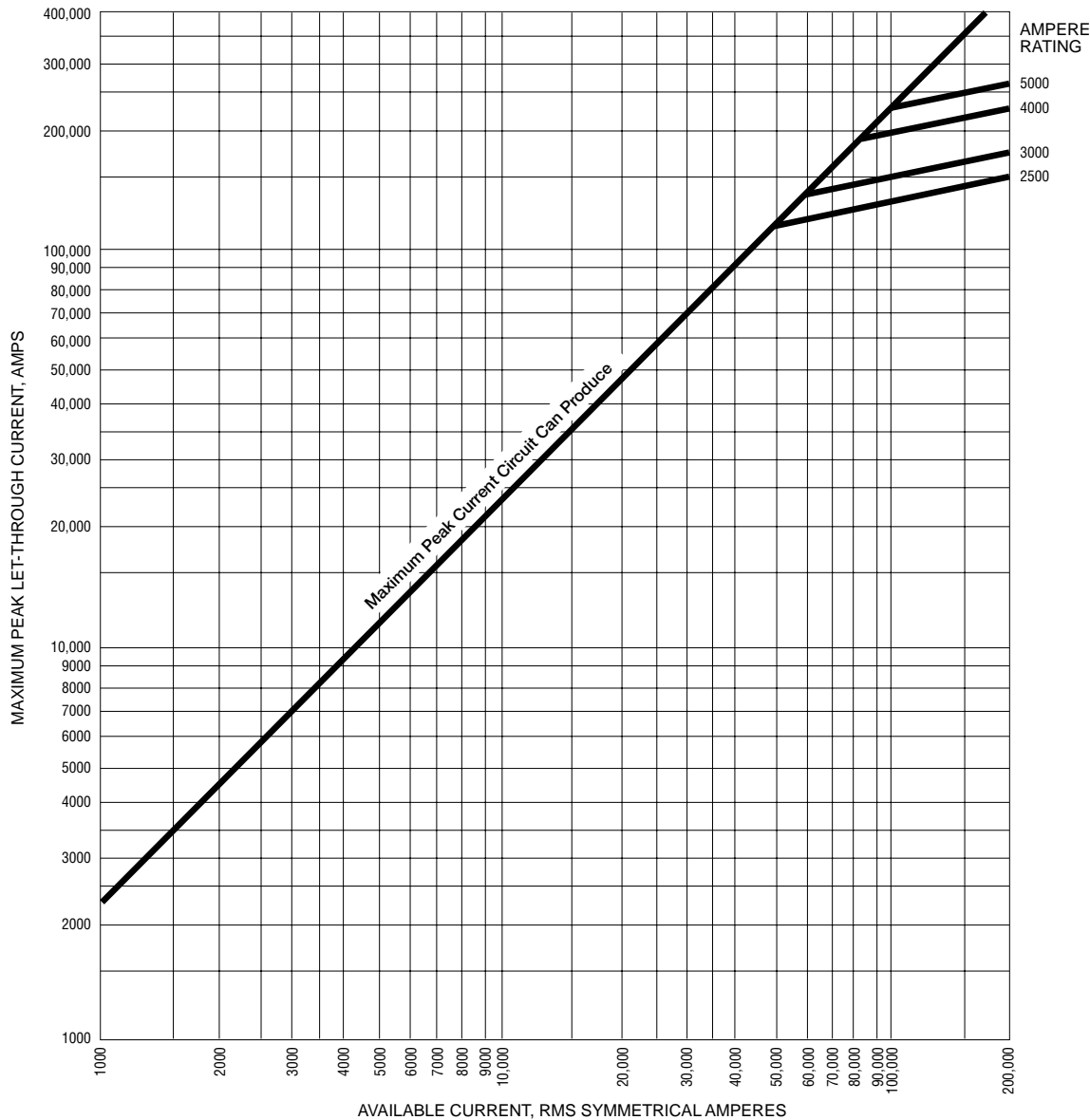
DSLII-632 and DSLII-840 Let-Through Characteristics
