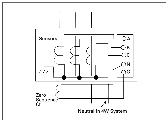
Sketch 2. Zero Sequence Feeder Breaker
