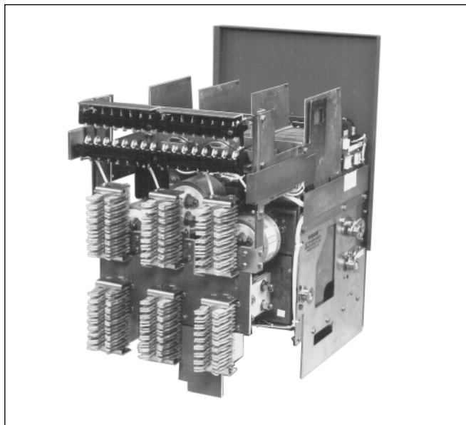
DSLII-620 Rear View
