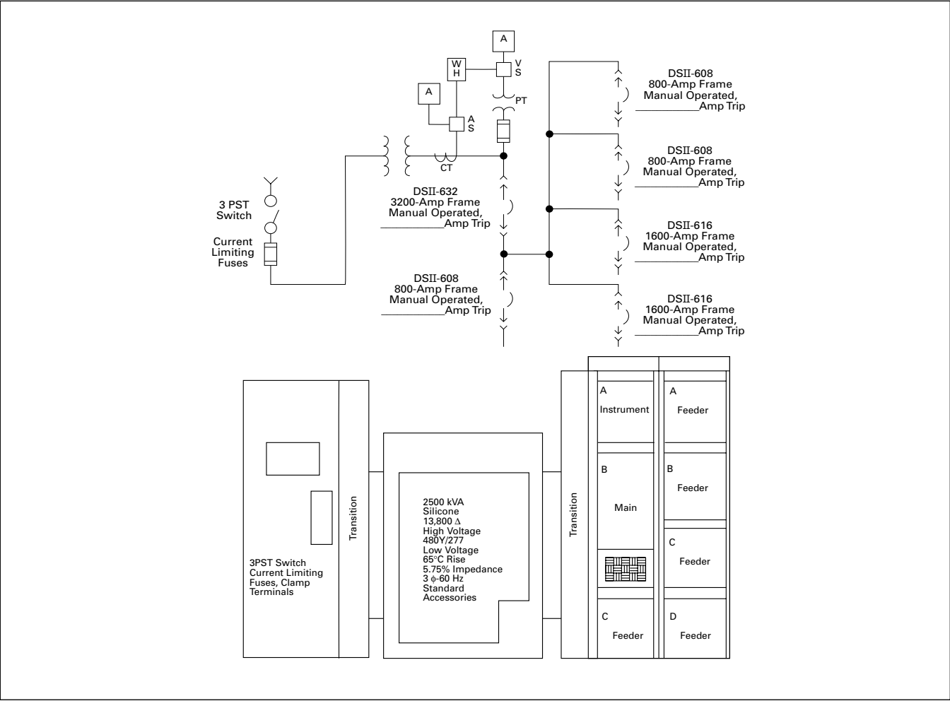
Single Line Diagram and Elevation
