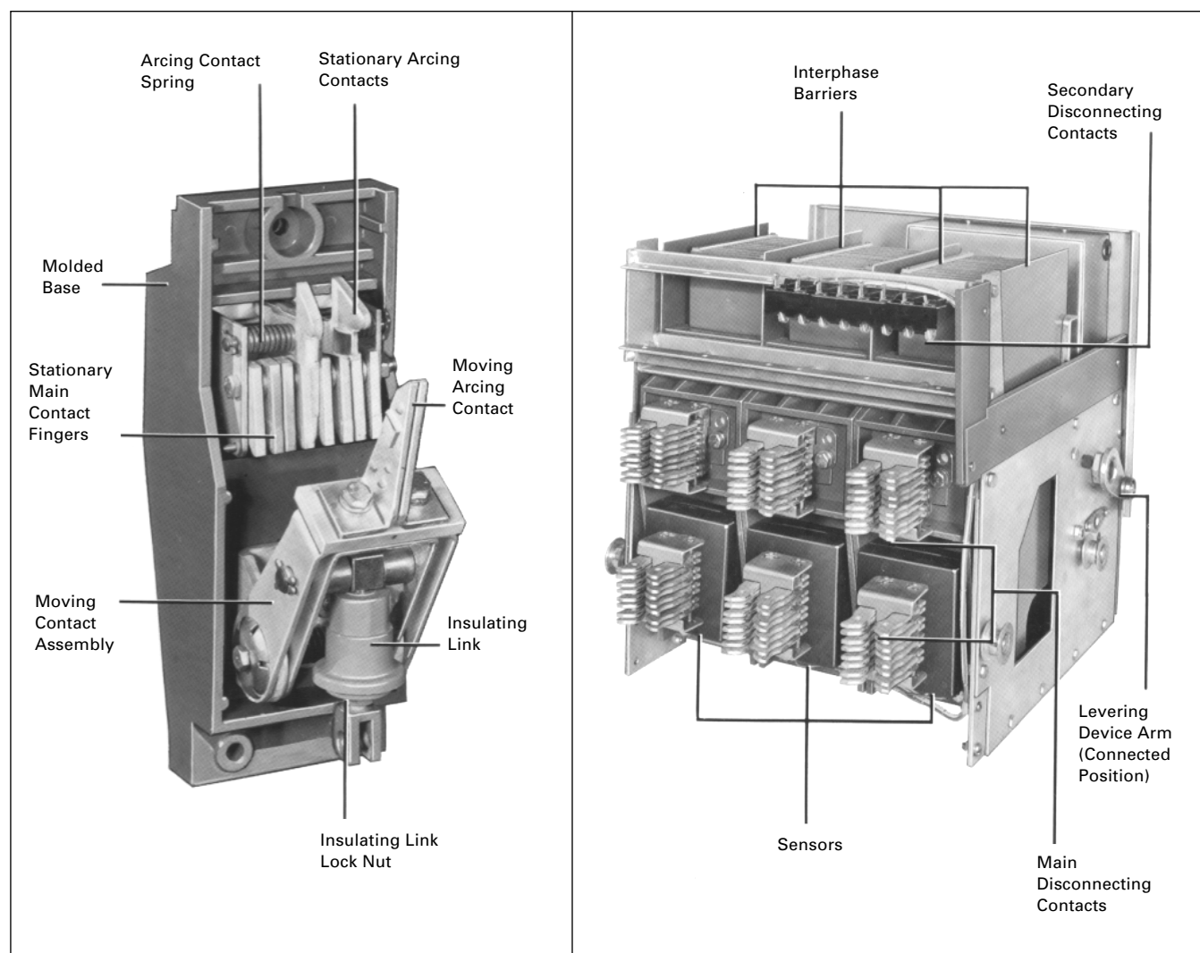
DSII Breaker Pole Unit
