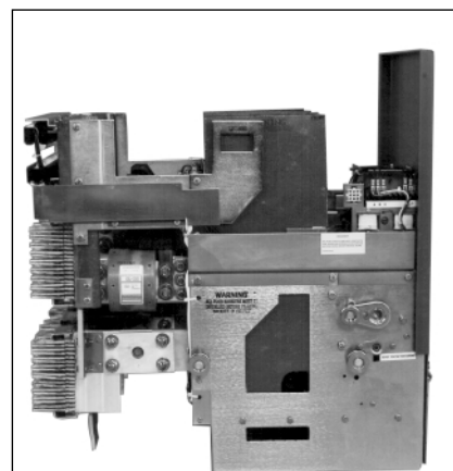
DSII Breaker Faceplate
