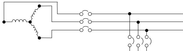
Figure 2. Three-Wire Distribution, Wye Source (Ungrounded)
