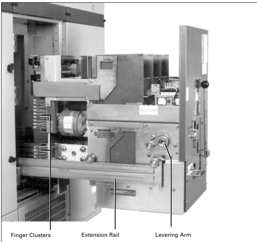
DSII Breaker on Extension Rails
