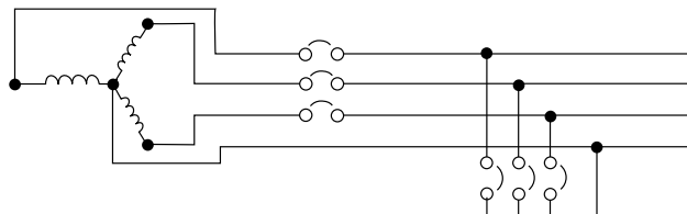
Figure 3. Four-Wire Distribution
