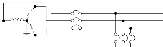
Figure 4. Three-Wire Distribution, Solidly Grounded System
