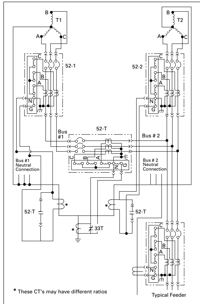
Sketch 5. Four-Wire Double-Ended Unit Substation
