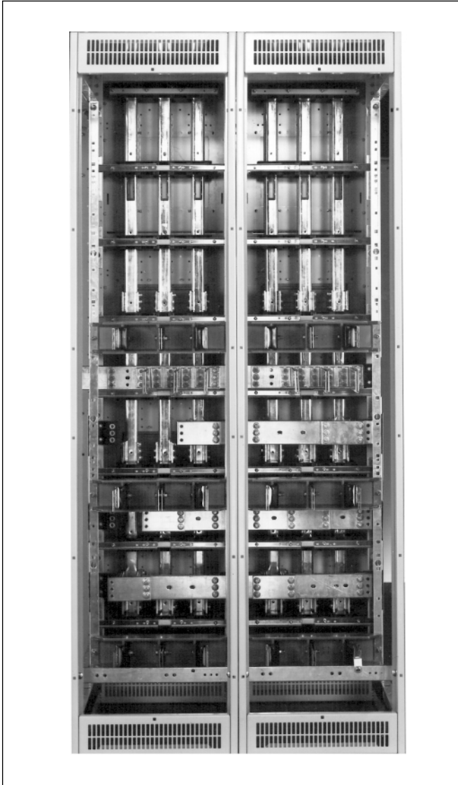
Bus and Cable Compartment with Barriers Removed
