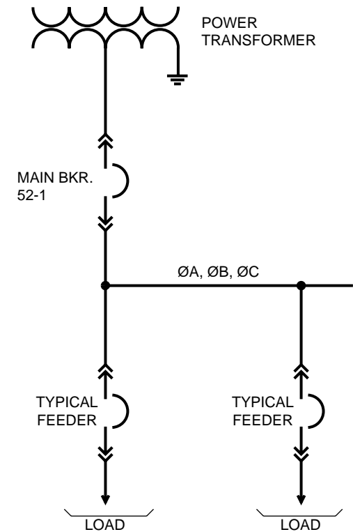
FIG. 7 SINGLE LINE DIAGRAM OF SWITCHGEAR
