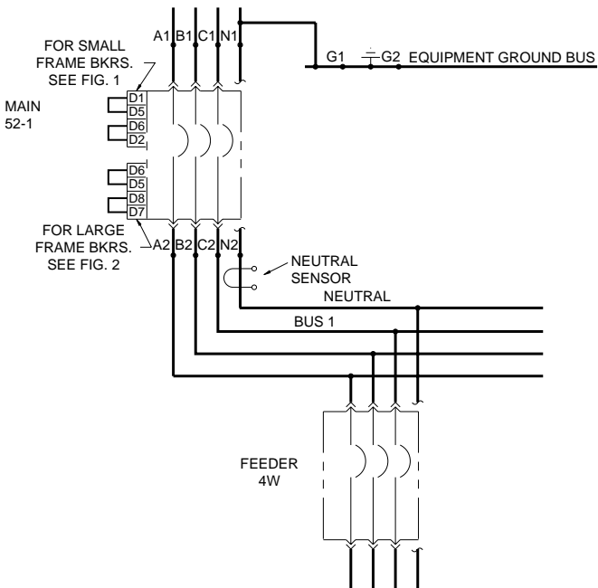
FIG. 10 THREE LINE DIAGRAM INDICATING TEST POINTS
