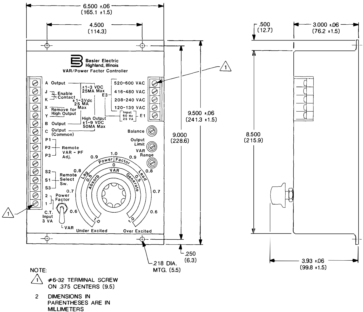
FIGURE 4 - OUTLINE DRAWING
