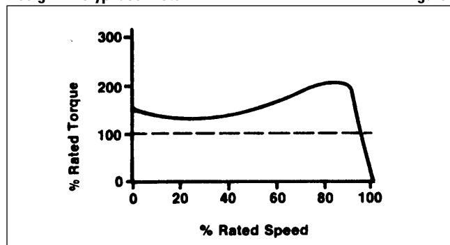
Design B Polyphase Motor
