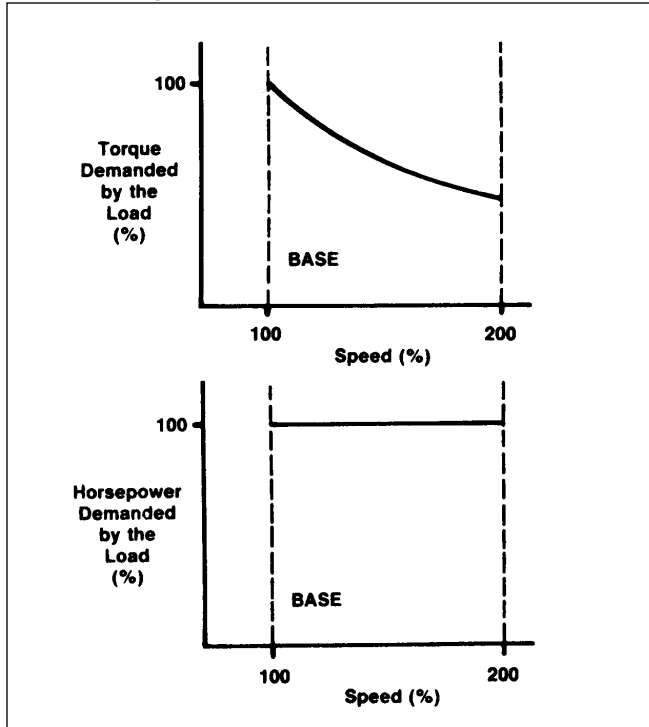
Constant Horsepower Load
