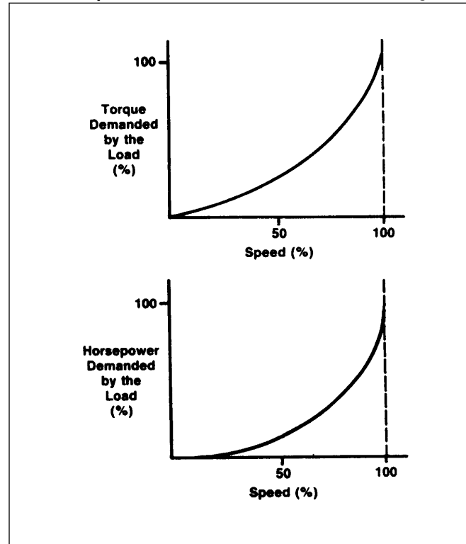
Variable Torque Load
