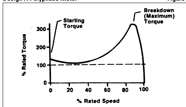
Design A Polyphase Motor
