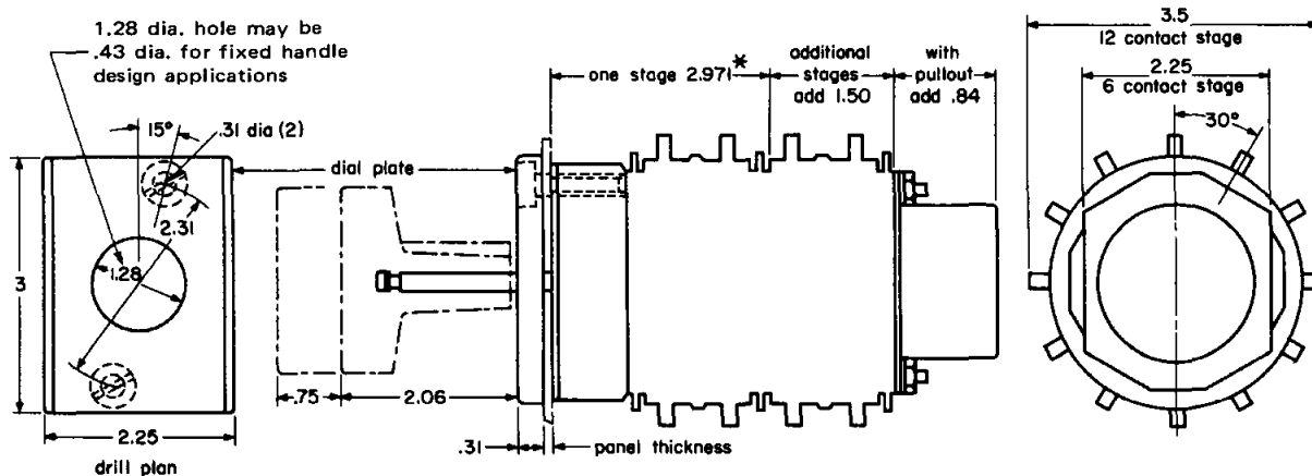
Fig. 2 Drilling Plan & Outline Dimensions of Standard W-2 Switches
